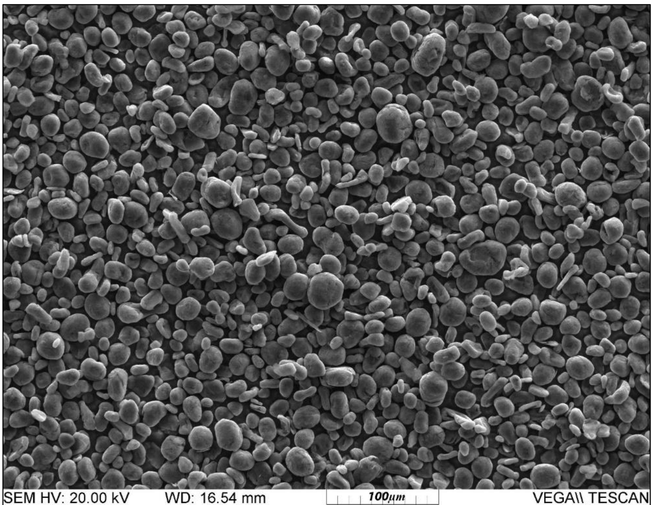
Image 5: Scanning Electron Microscope (SEM) image of Lac Rainy purified spherical graphite (average 19µm)
