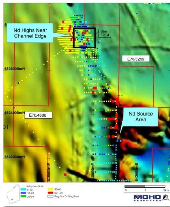
Figure 15: Neodymium distribution in soils in magnetics (TMI) on E70/5154 and E70/4688 at 865300 Burracoppin
