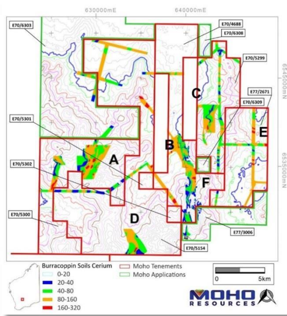
Figure 13: Distribution of cerium in soils at Burracoppin Project
