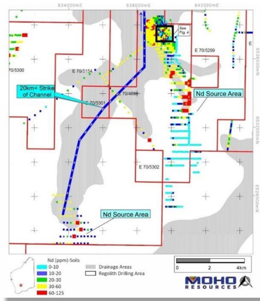
Figure 14: Neodymium distribution in soils in relation to interpreted drainage channels on E70/5154 and E70/4688 at Burracoppin
