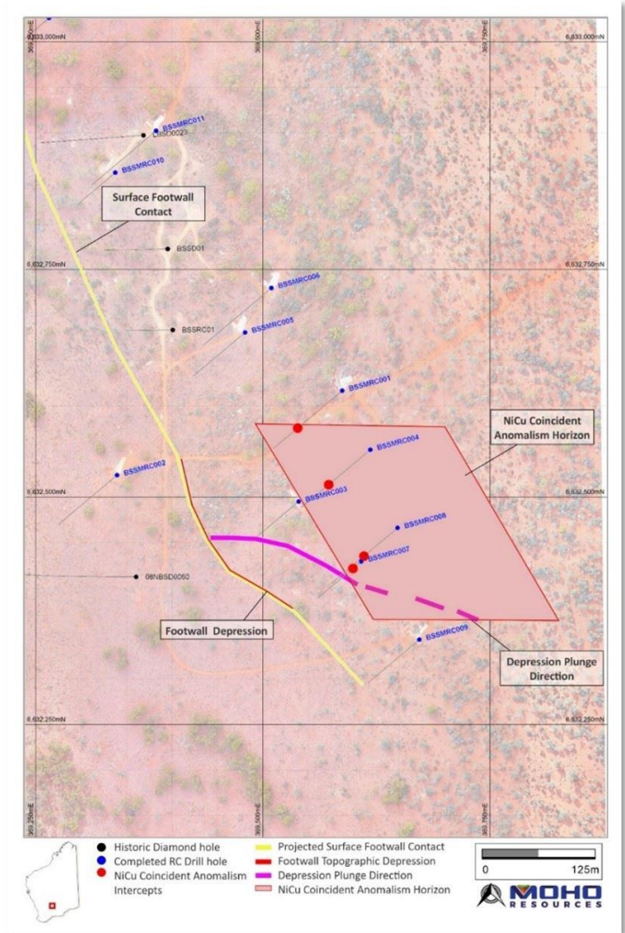
Figure 20: Coincidental Ni-Cu anomaly horizon intersected in RC drilling
