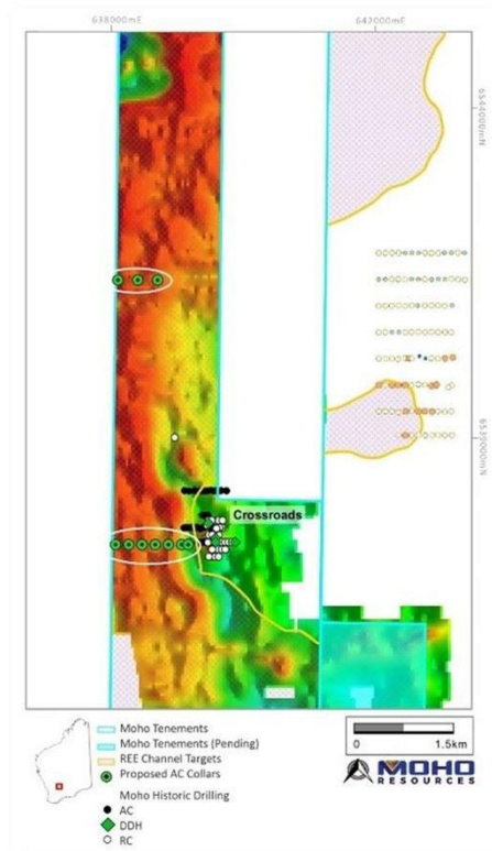
Figure 11: Location of lines of air core drill holes on Background - AEM survey (2018) with interpreted channel
