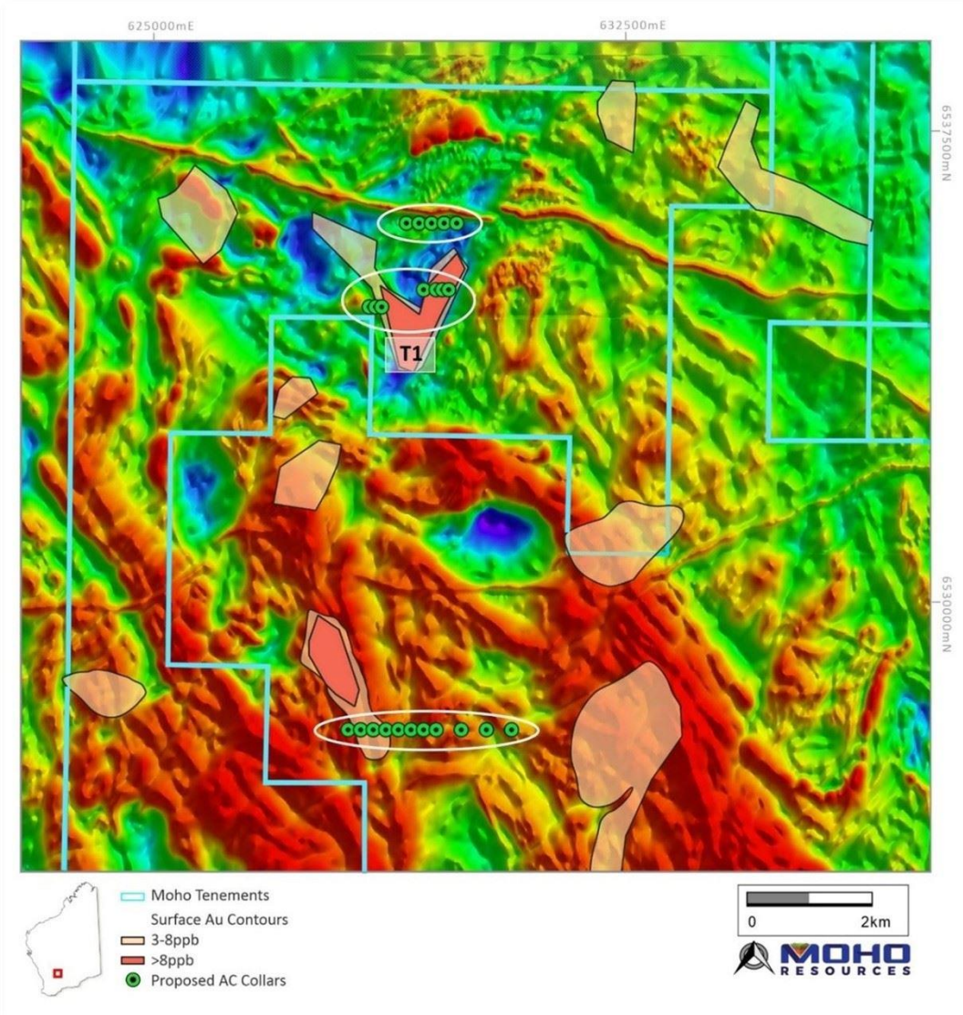
Figure 12: Location of lines of proposed air core drill holes to investigate potential clay-hosted REE mineralisation and historic surface gold mineralisation on E70/5300 and E70/5154
