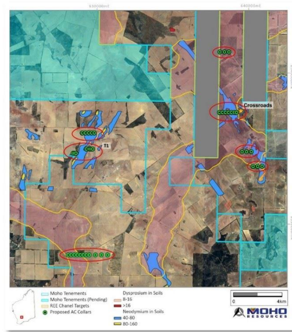
Figure 10: Proposed air core drill holes in relation to areas E70/4688 in elevated Dysprosium and Neodymium
