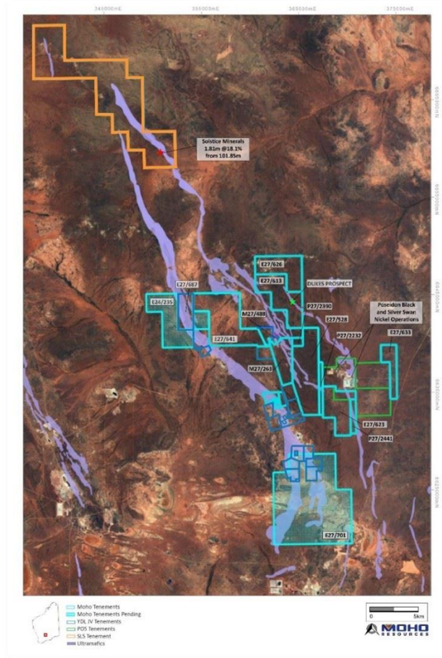
Figure 16: Location of Dukes nickel prospect at Moho’s Silver Swan North Project in relation to ultramafic geology mapped by GSWA
