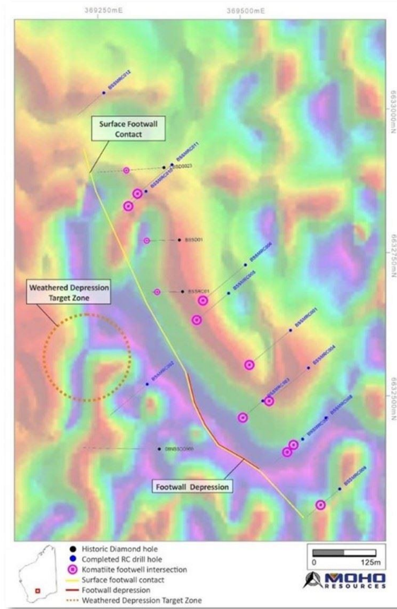
Figure 18: Drill Hole location plan
