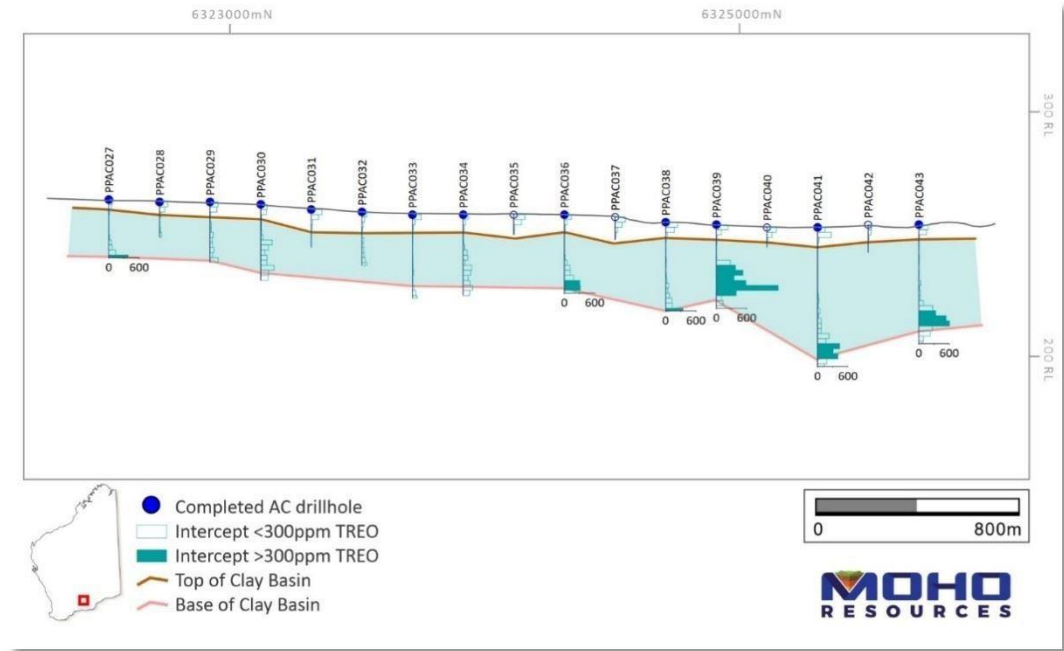
Figure 4: Ned's Corner Road Prospect Aircore Drillhole Section. (Vertical exaggeration 10X)
