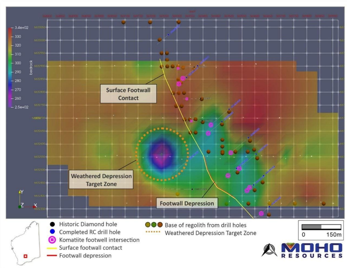
Figure 21: Passive seismic survey plan
