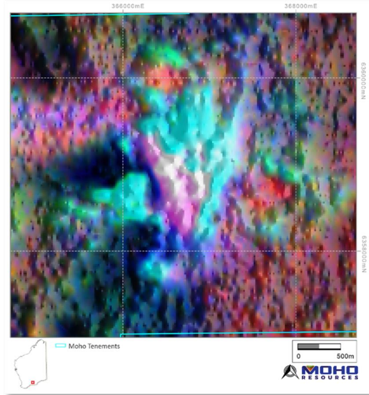
Figure 5: Ternary image of radiometrics (potassium - red, uranium - blue, thorium - green) overlain on shaded relief from Dose Rate
