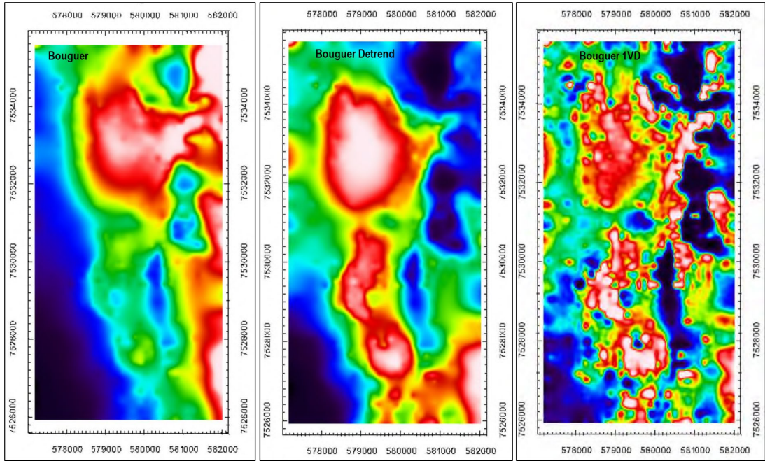
Figure 19: Gravity Image Bouguer, Bouguer Detrend, Bouguer 1VD.
