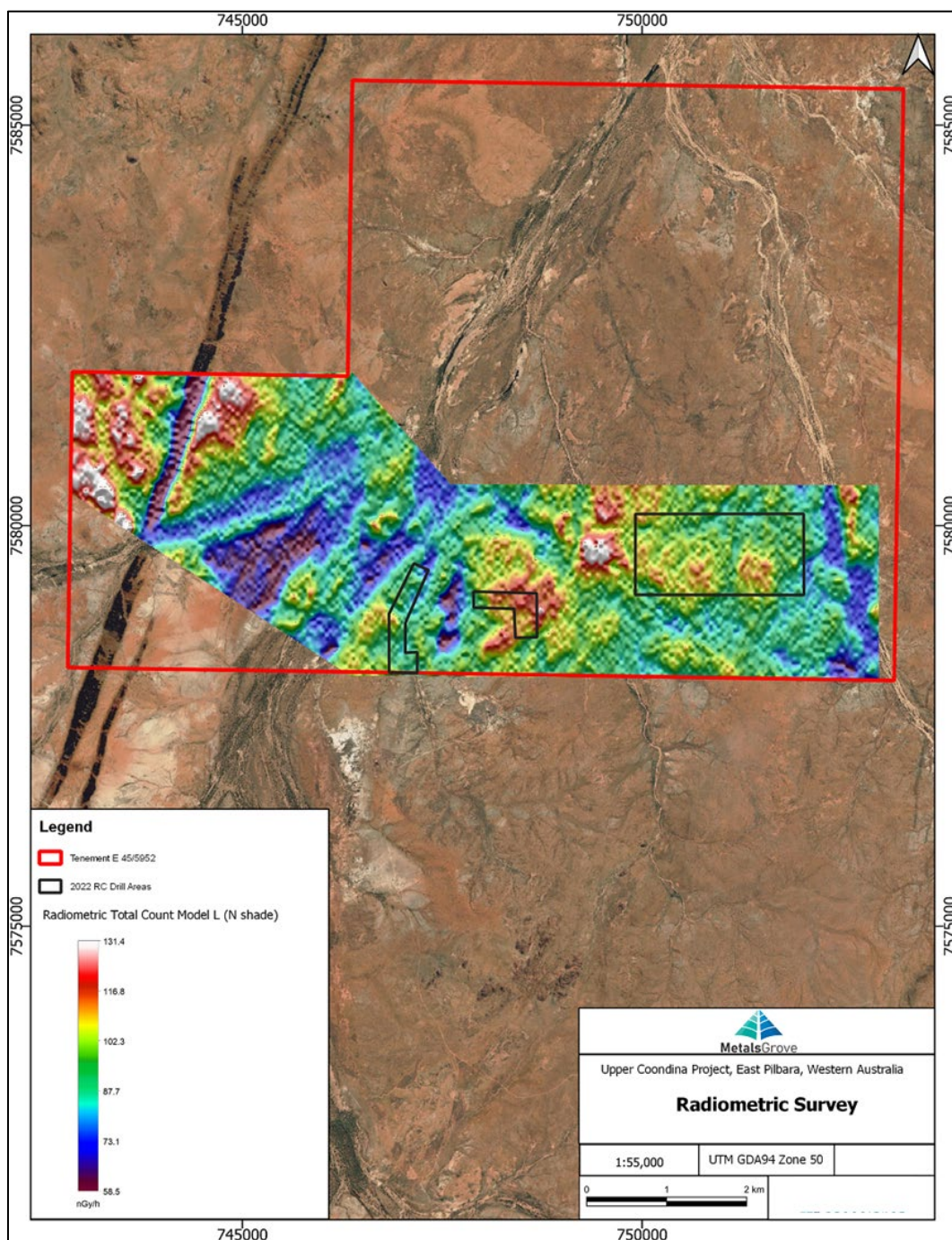
Figure 26: Radiometric total count model with north shade.
