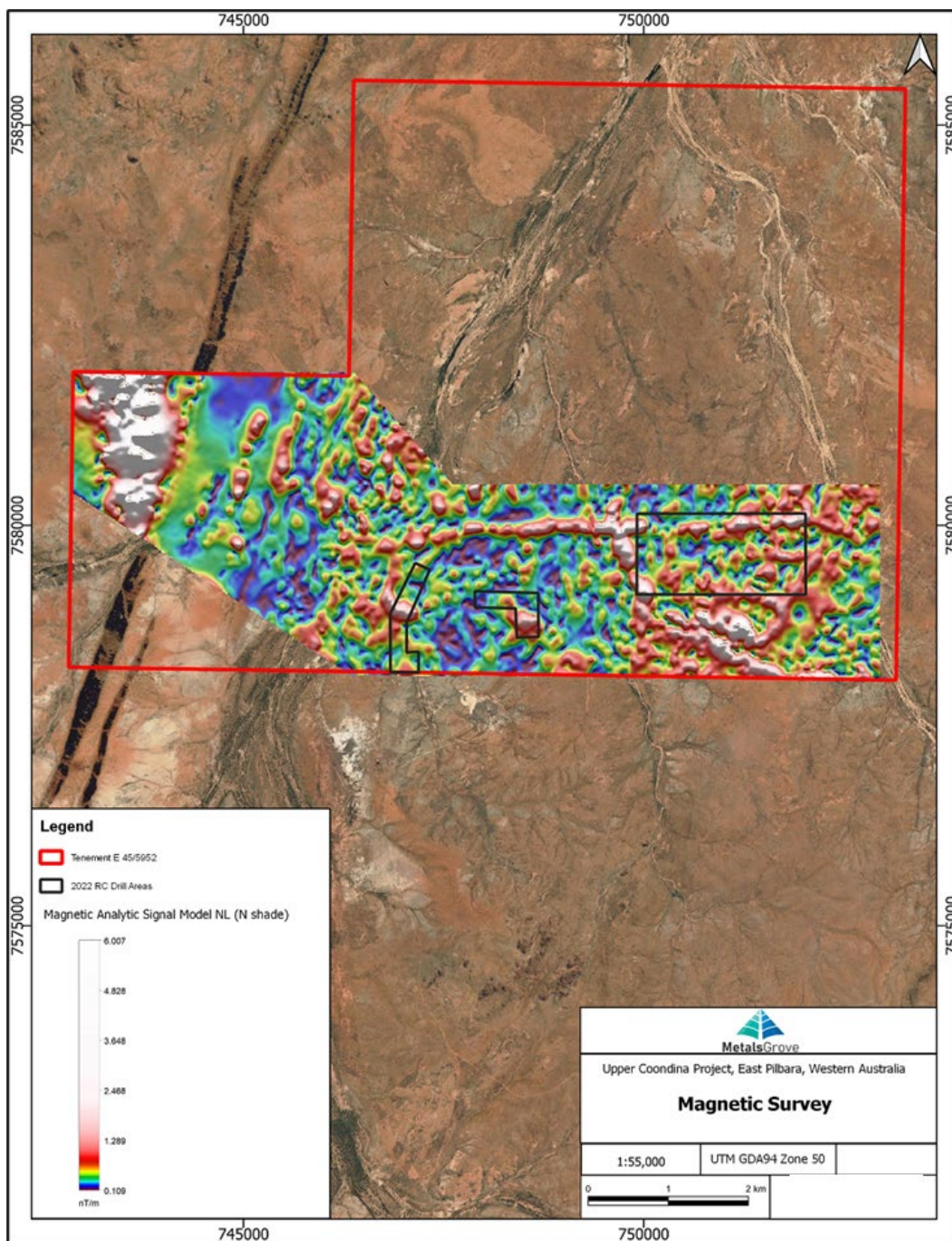
Figure 25: Magnetic analytic signal model with north shade.
