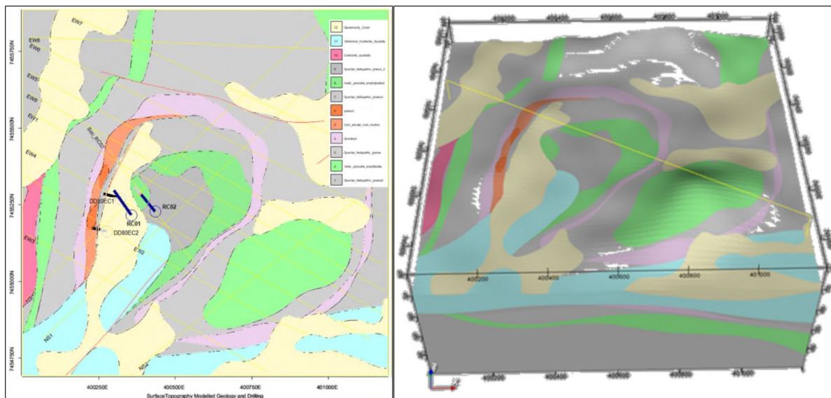
Figure 15: Implicit 3D Volumetric Geological Model.
