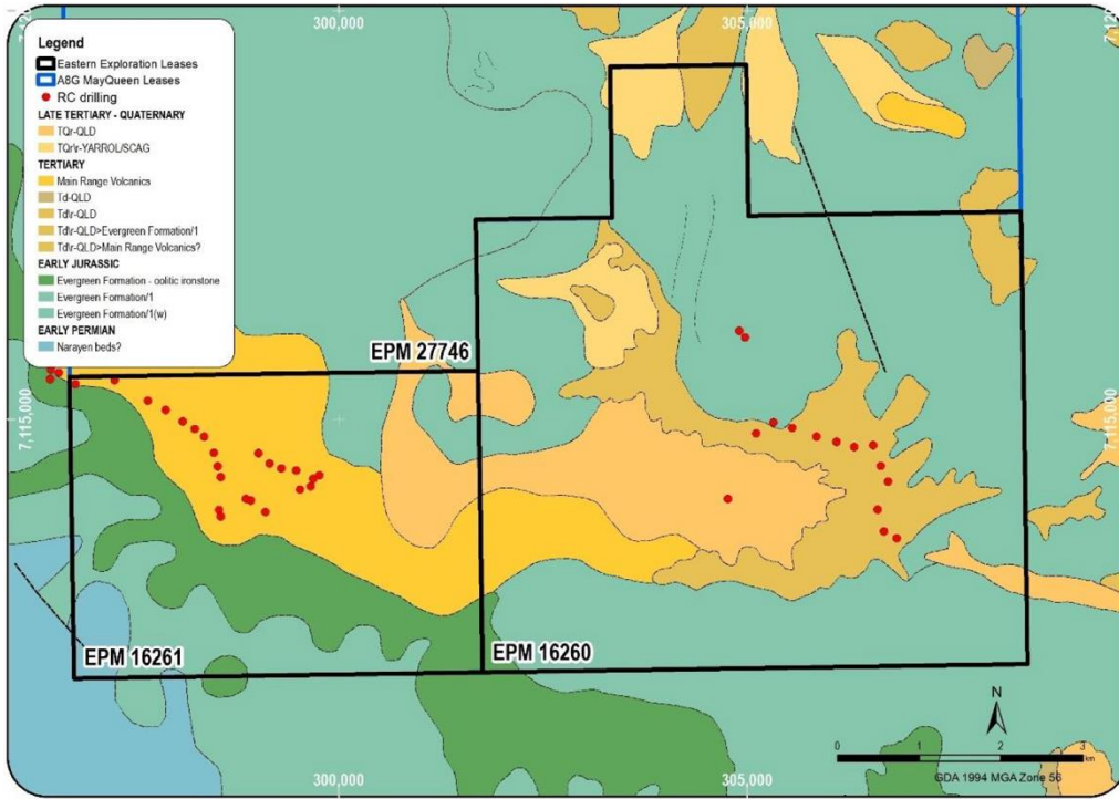
Figure 8: Basic geology of the EPM16260 and EPM 16261 with RC hole's locations marked
