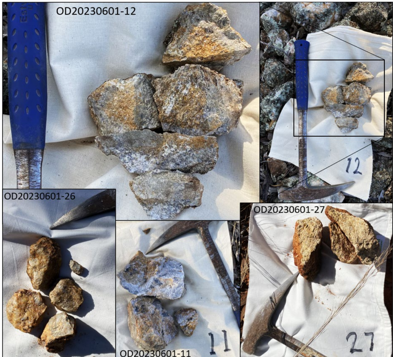
Figure 12: Narriah Project – Photos of key rock chip samples, descriptions starting at the top left and moving counterclockwise: OD20230601-12: Micaceous quartz-eye Erigolia Granite with pale grey bands of possible xenoliths (grading 0.16% Li 2 O ). OD20230601-26: Quartz veining with 5mm cassiterite crystals and elongated wolframite and tourmaline crystals (grading 3.59% Tin and 0.63% Tungsten ). OD20230601-11: Quartz blow with wolframite and minor granite wall rock (grading 0.11% Tin and 1.66% Tungsten ). OD20230601-27: Weathered micaceous granite from mullocks with less abundant quartz-eyes and greener tinge possibly indicating less weathering (grading 0.16% Li 2 O ).
