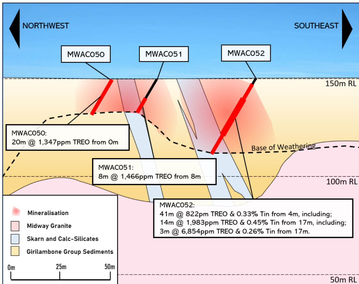
Figure 11: Doradilla Project – Cross-section from MWAC050 to MWAC052 showing the multiple skarns of the DMK line associated with REE and tin mineralisation above the Midway Granite which underlies the area.
