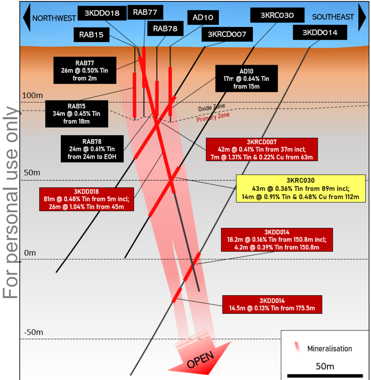
Figure 8: 3KEL Target – Cross section of 3KRC007, 3KDD014, 3KDD018 and recent hole 3KRC030, recent results are in yellow.
