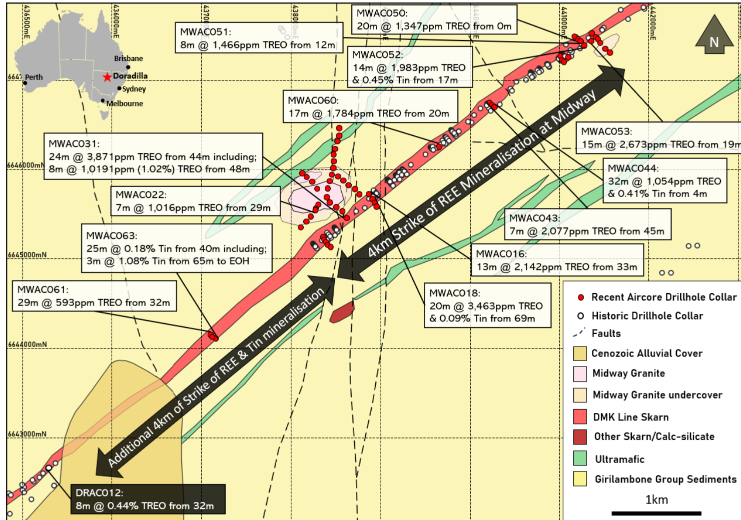
Figure 9: Doradilla Project – Map shows the large strike extension of the previously undrilled and untested strike between Midway and Doradilla on the DMK Line and the previous strike extent with recent aircore drilling intercepts overlaid on the mapped and interpreted geology.
