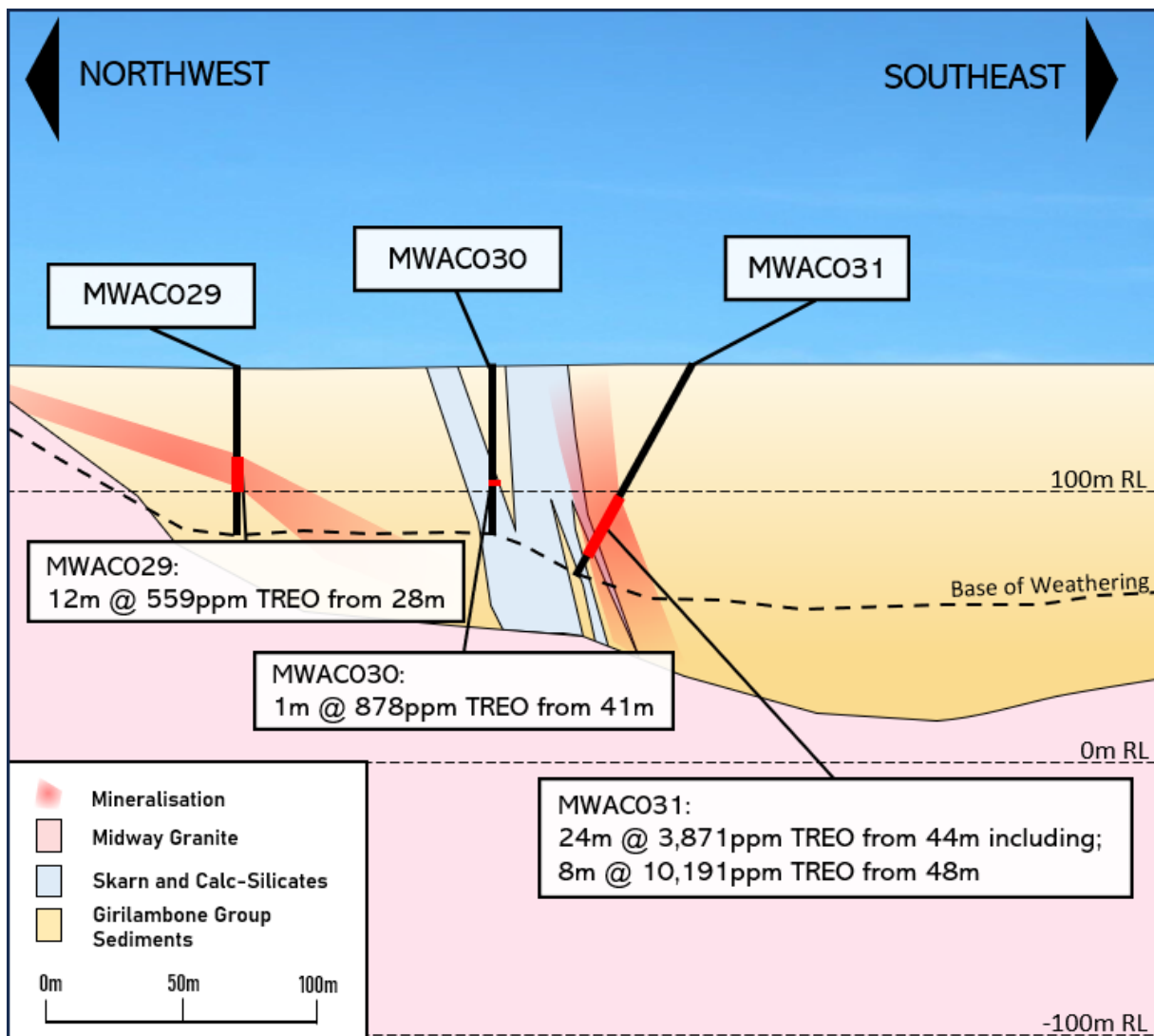
Figure 10: Doradilla Project – Cross-section from MWAC029 to MWAC031 showing the DMK line Skarn above the Midway Granite with the Midway Granite coming to surface and outcropping to the northwest.
