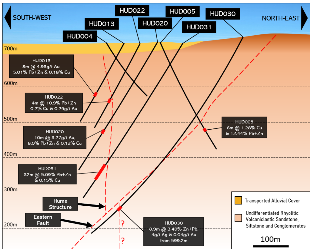
Figure 13: Hume Target – Cross-section of HUD030 showing the trace in red of the extension of the hole to test the Hume Structure at depth and provide a platform for DHEM – Assays are pending for the extended hole interval shown in red.
