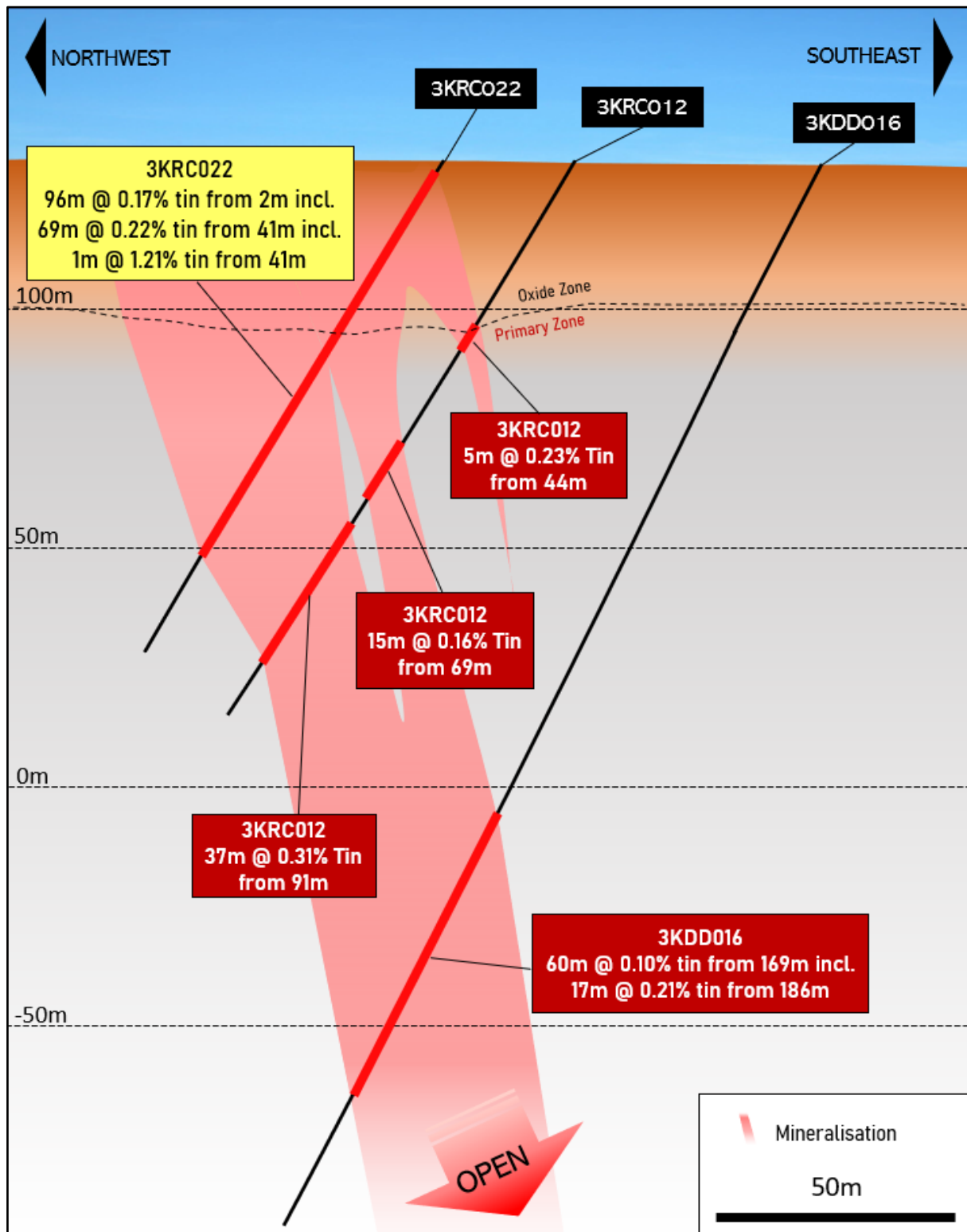
Figure 6: 3KEL Target – Cross section of 3KRC012, 3KDD016 and recent hole 3KRC022, recent results are in yellow.
