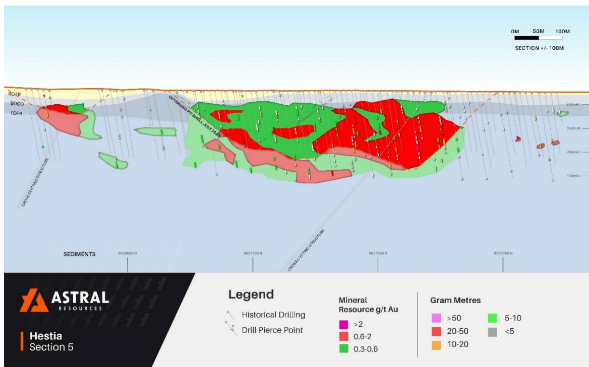
Figure 10 – Hestia long projection view (refer Figure 5 for section location)
