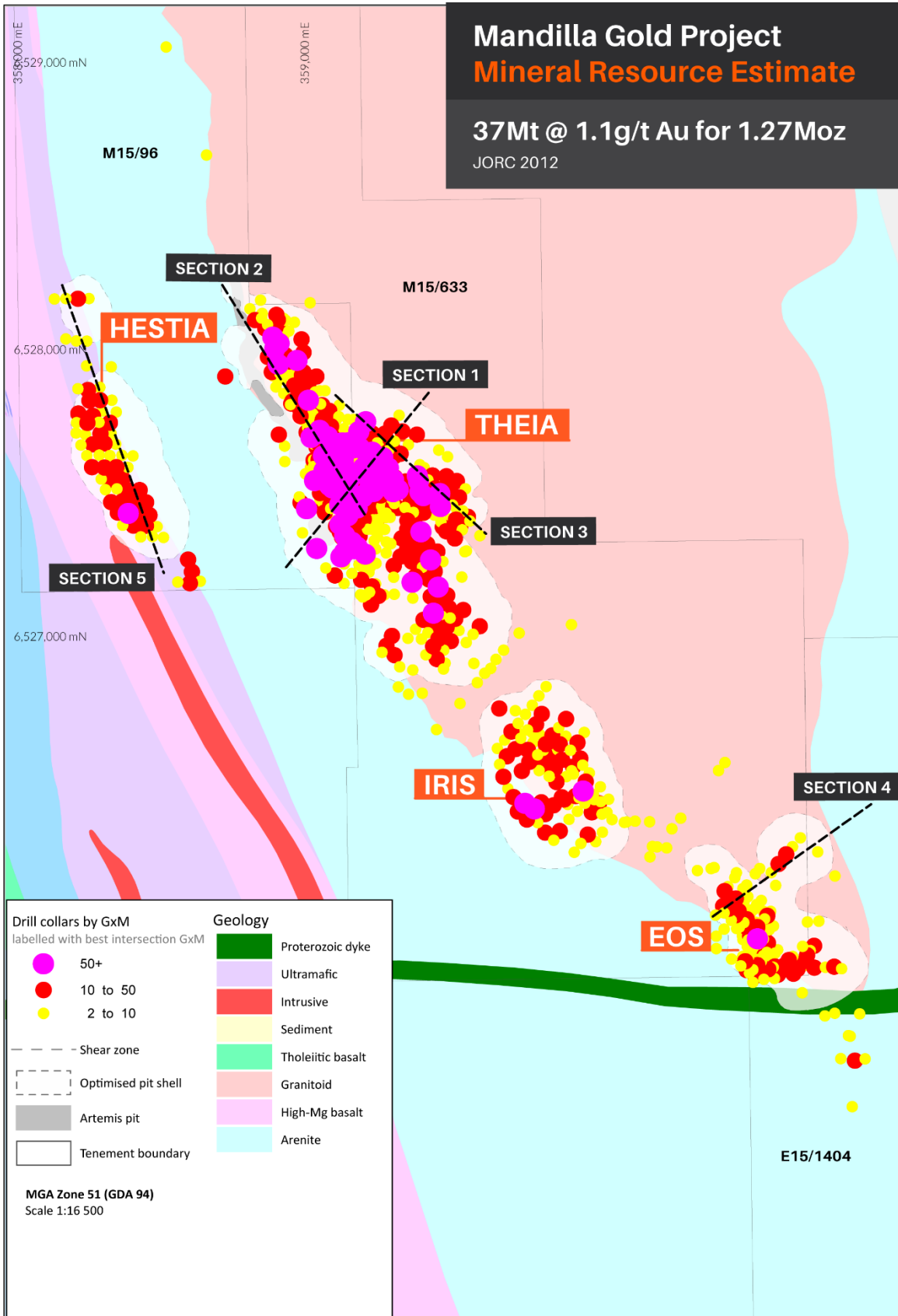
Figure 5 – July 2023 MRE optimised pit shell and section locations on local area geology.
