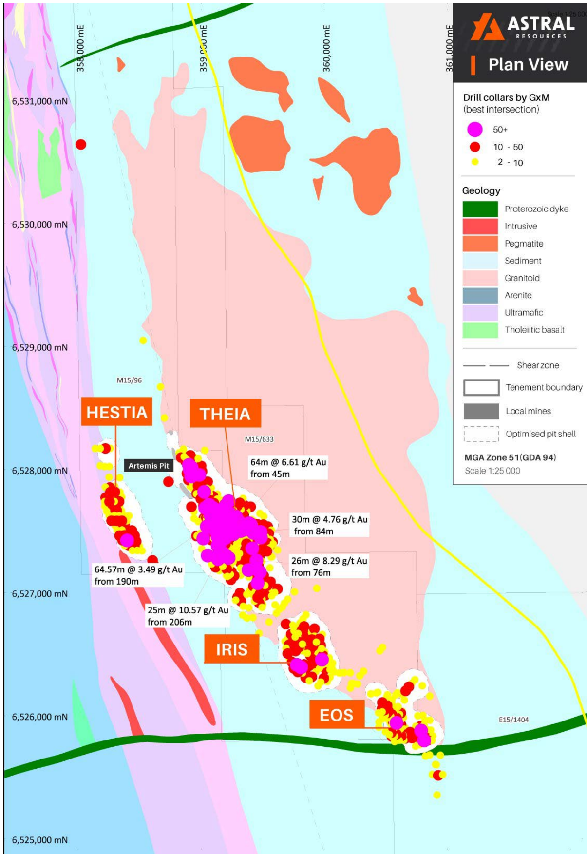
Figure 3: Mandilla Local Area Geology (including significant recent intercepts).
