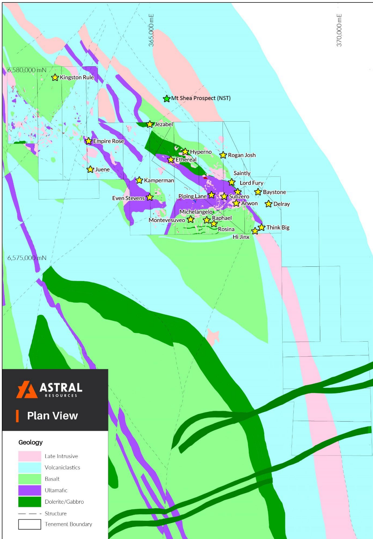
Figure 11 – Feysville Gold Project showing tenements and deposits prospects on local area geology.
