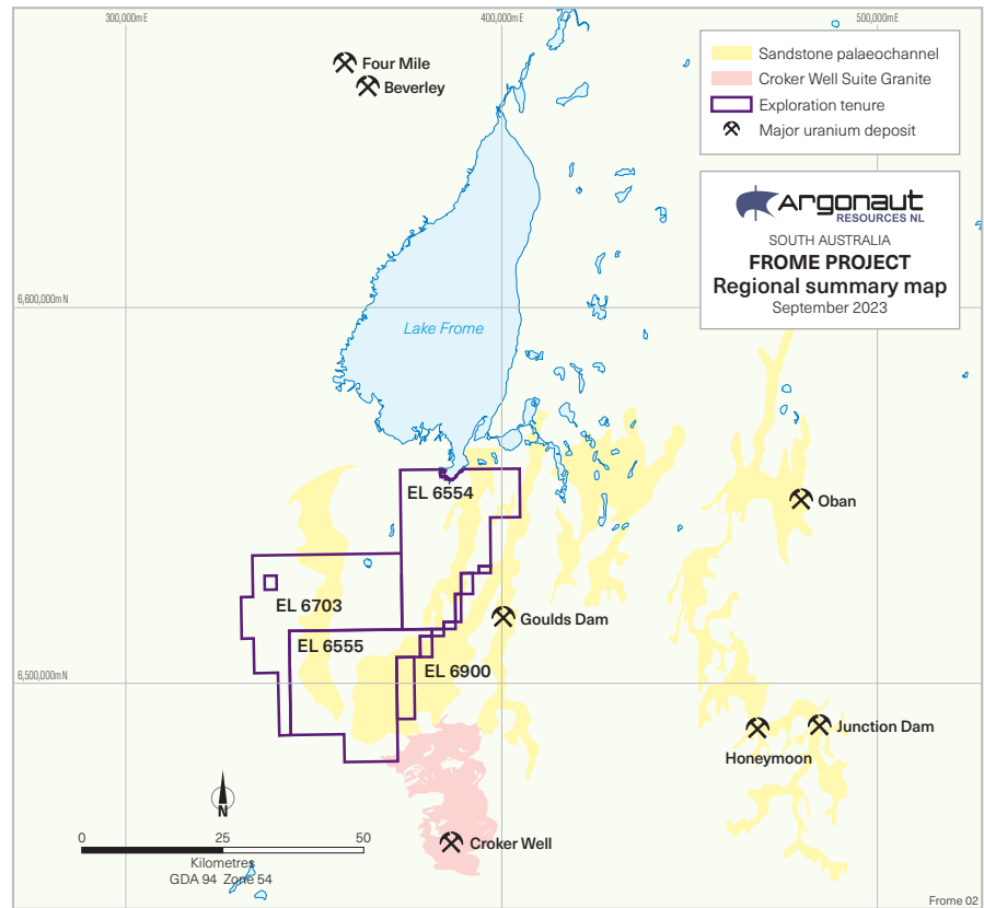
Figure 2 Frome project tenement locations and major uranium deposits
