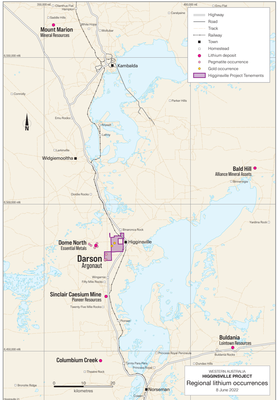
Figure 8 Regional lithium pegmatite deposits in the area of the Darson Pegmatite Swarm, Higginsville, WA.
