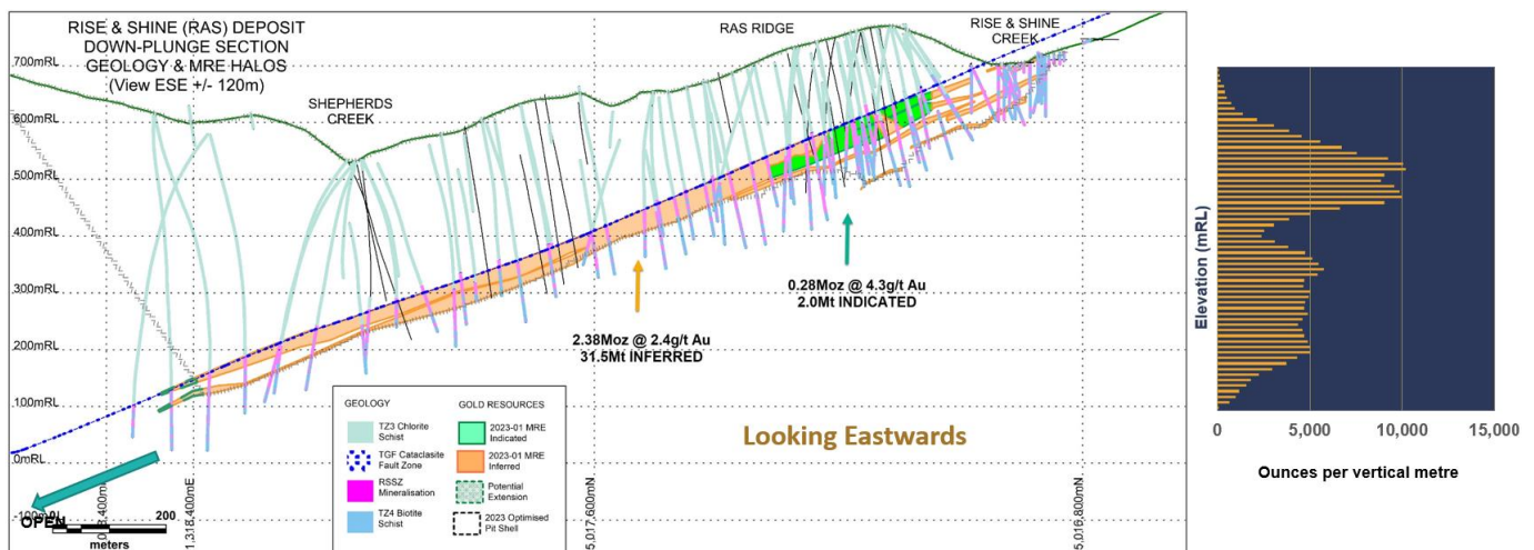
Figure 5 - Long section through RAS looking east with the ounces per vertical metre aligned with elevation.
