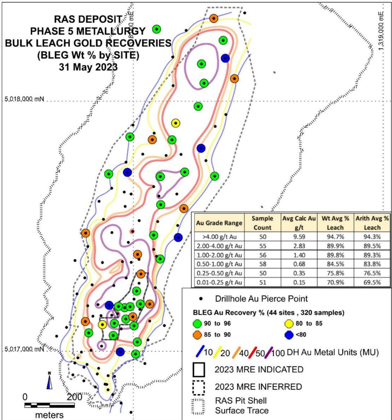
Figure 6 Location of BLEG samples and their respective gold recovery via cyanide leach
