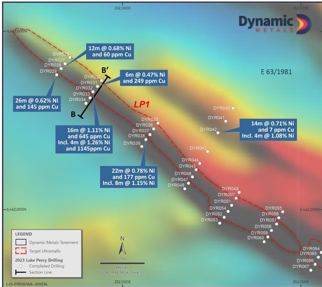
Figure 8. Plan view of drill collar positions at LP1 and significant assay results against magnetic background
