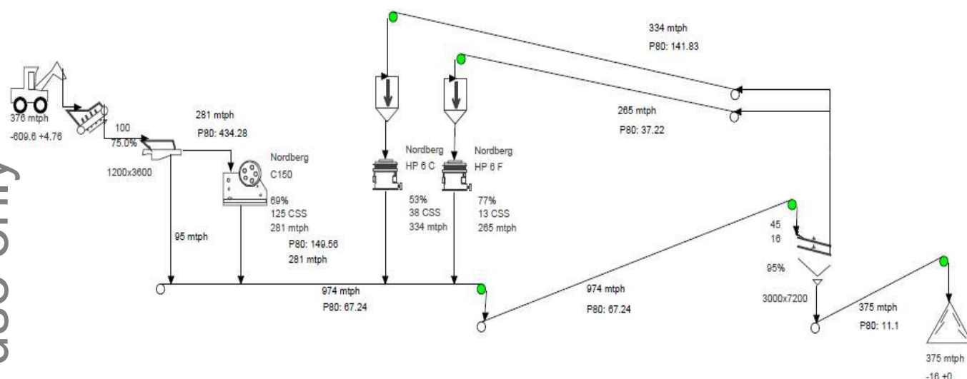
Figure 23 – AggFlow model of the three-stage crushing circuit
