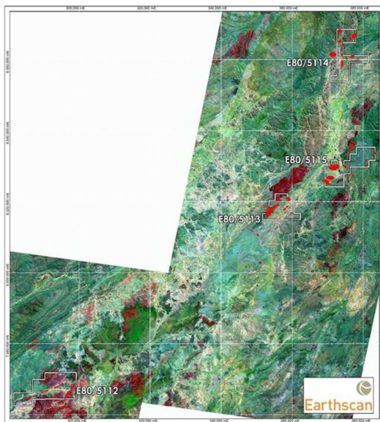
ASTER TARGETS OVER ASTER BANDS 731
