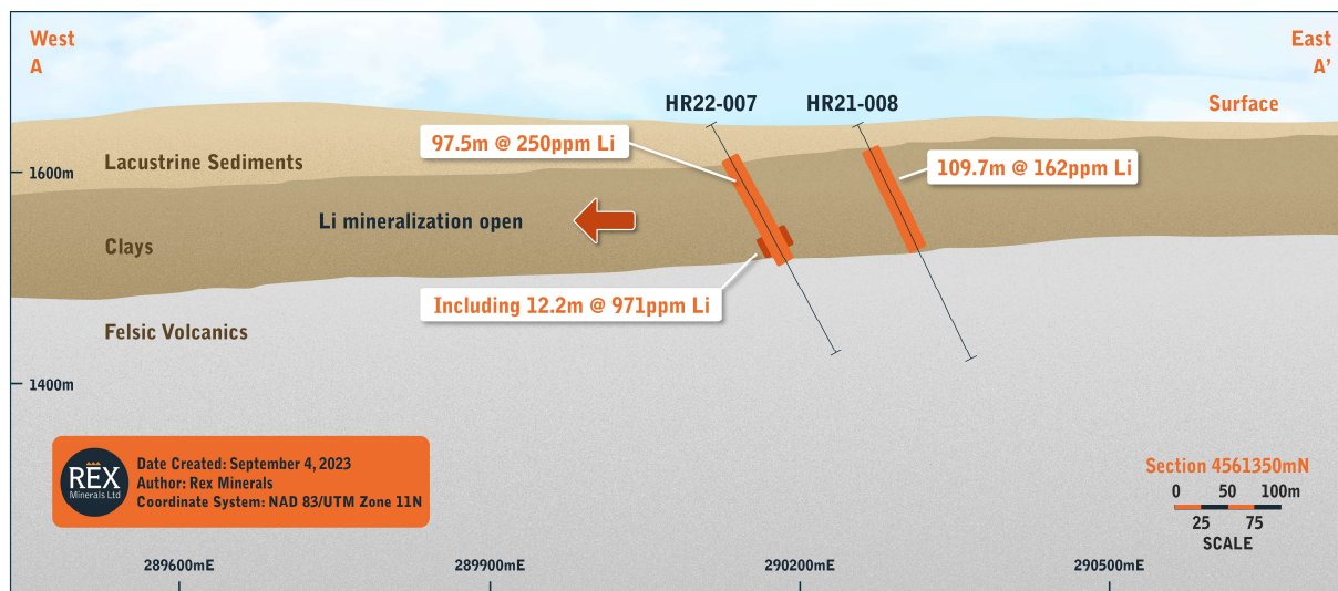
Figure 5: Cross section illustrating anomalous Li values at the Airport project. Drill hole HR21-008 contains elevated lithium concentrations that exceed 100ppm Li. Lithium contents increase to the west in drill hole HR22-007 (including an intersection of 12.2m @ 971ppm Li) with increasing proximity to the centre of the caldera.
