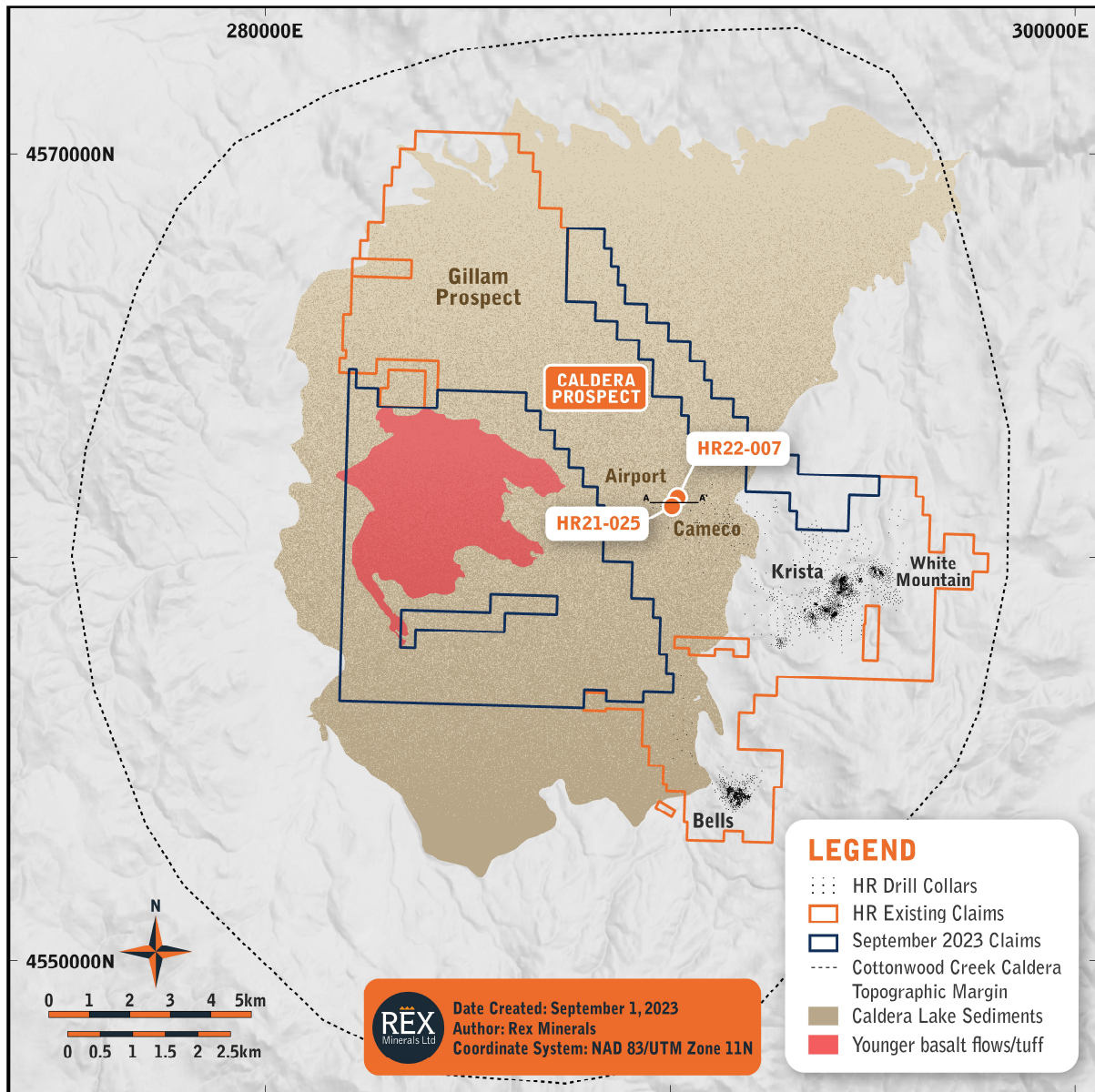
Figure 4: Geology map highlighting the new mining claims (blue) which cover the prospective area for lithium mineralisation at Hog Ranch.
