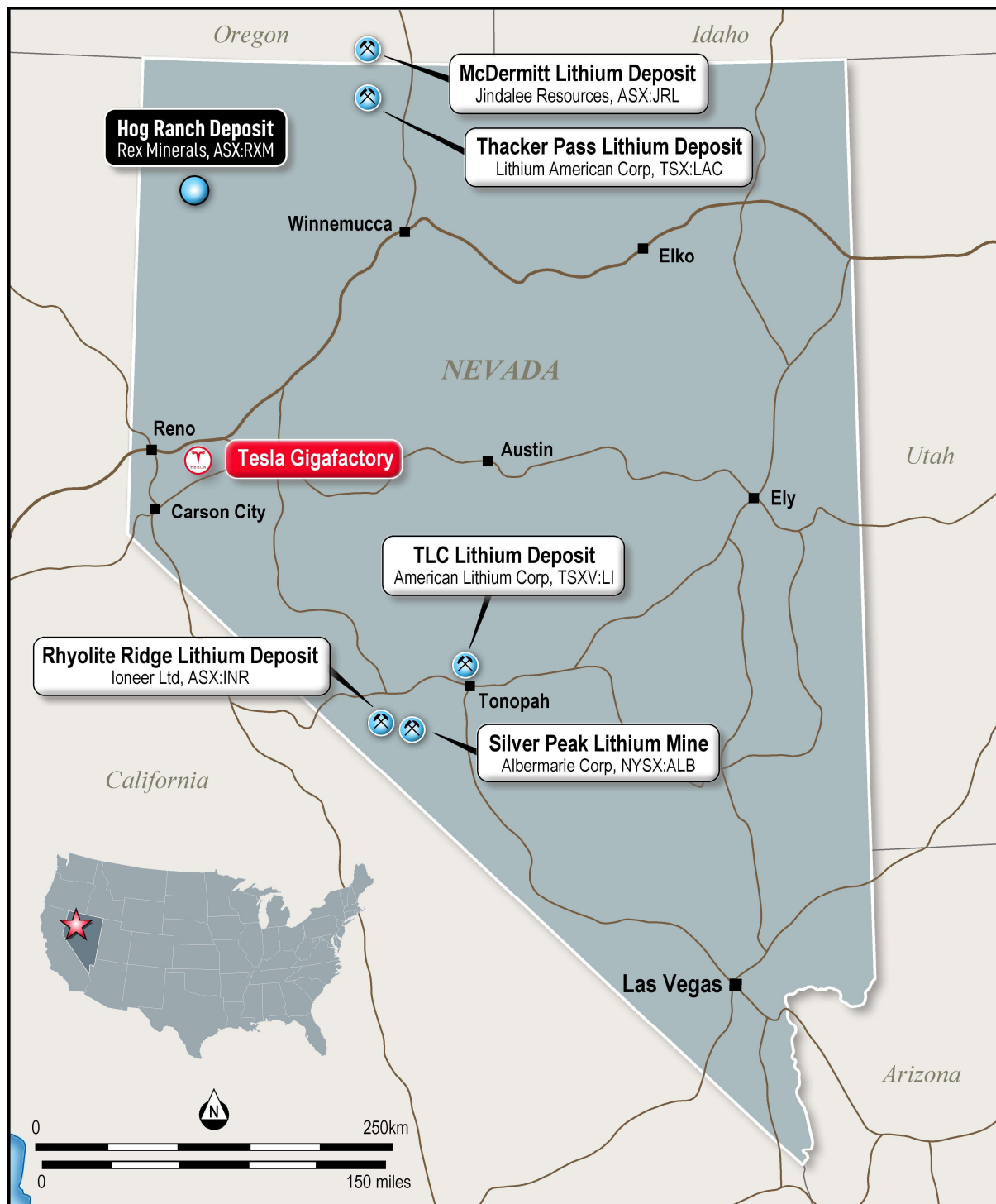
Figure 1: Location of significant lithium deposits throughout Nevada relative to Hog Ranch.
