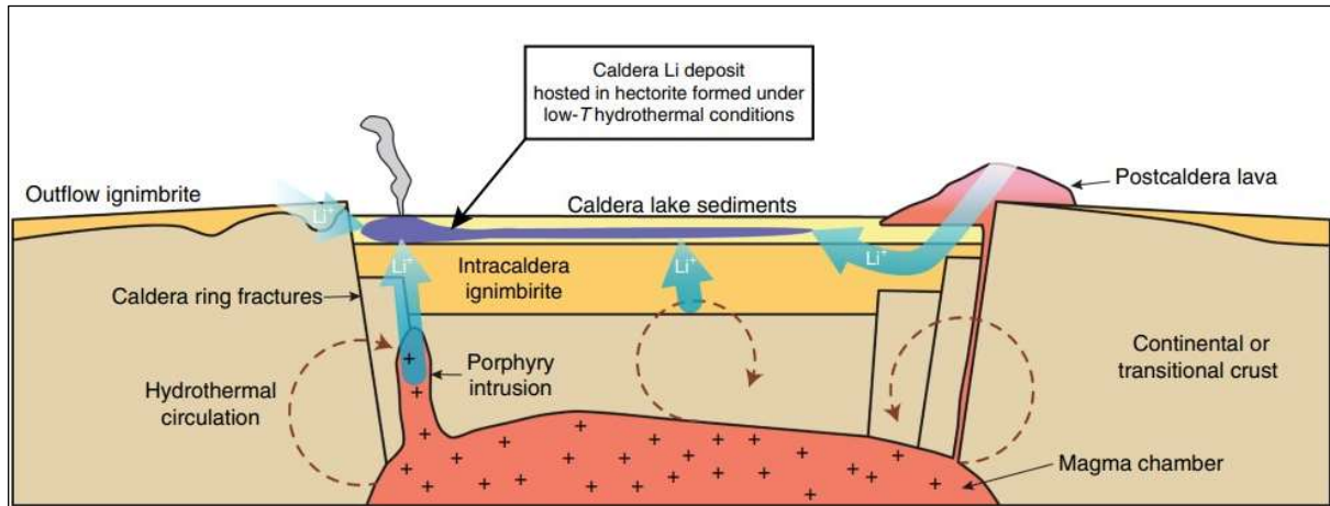
Figure 3: Schematic diagram highlighting the interpreted mode of formation of caldera-hosted Li Clay deposits similar to the geological setting at both the McDermitt Caldera (host to Thacker Pass) and the Cottonwood Creek Caldera (host to the Lithium mineralisation at Hog Ranch). From Benson, et. al., 2017.
