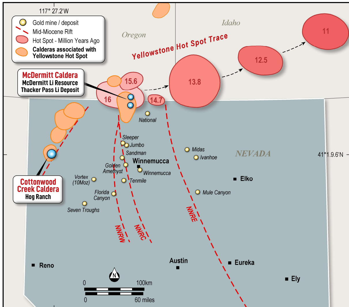
Figure 2: Location of Cottonwood Creek Caldera (host to Hog Ranch) and the McDermitt Caldera (host to Thacker Pass Li deposit) which are both large caldera systems which formed ~16 million years ago relating to the development of the Yellowstone Hotspot.
