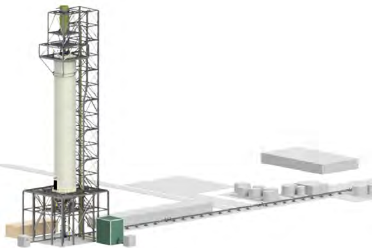
Depiction of a 3.1MW Calix electric calciner for a mid-stream lithium processing demonstration plant.
