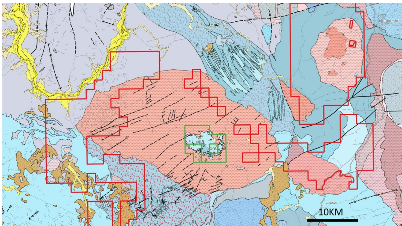
Figure 1 Torrington Project Geology. Granite batholiths are colored orange. GCM tenements outlined in Green encapsulate the Torrington metasedimentary roof pendant. FMG tenements outlined in Red.
