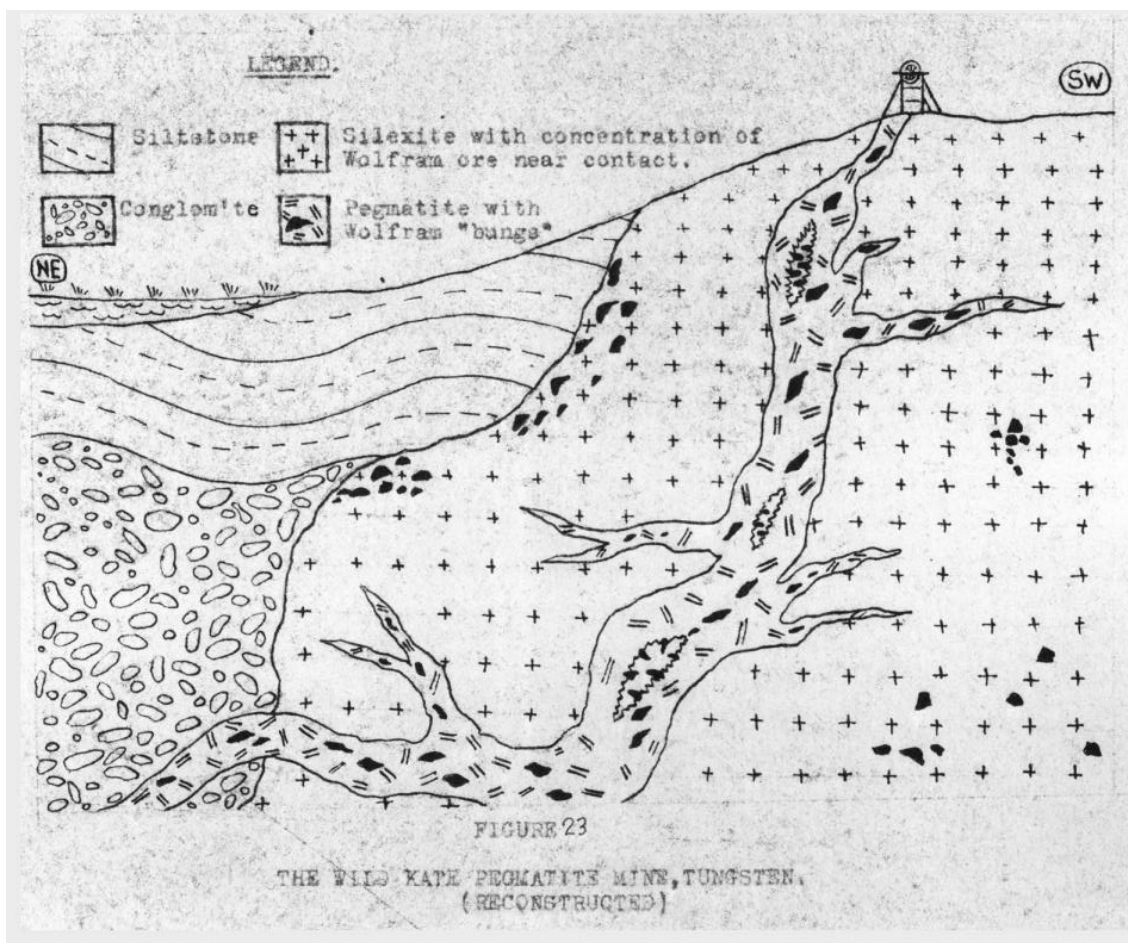
Figure 6 Wild Kate lithium and tungsten rich pegmatite
