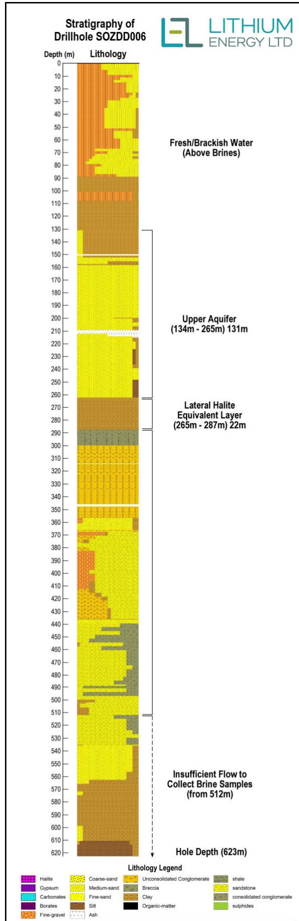
Figure 3: Drillhole Stratigraphy for SOZDD006
