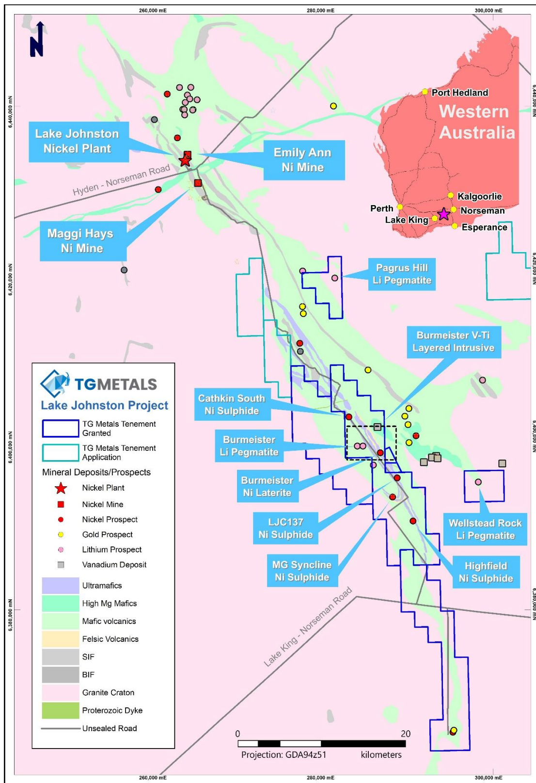
Figure 1 – Simplified Geology of the Lake Johnston Project with prospect locations Datum: AMG Zone 51 (GDA94). The dashed outline is the initial drilling area and lithium anomaly location.
