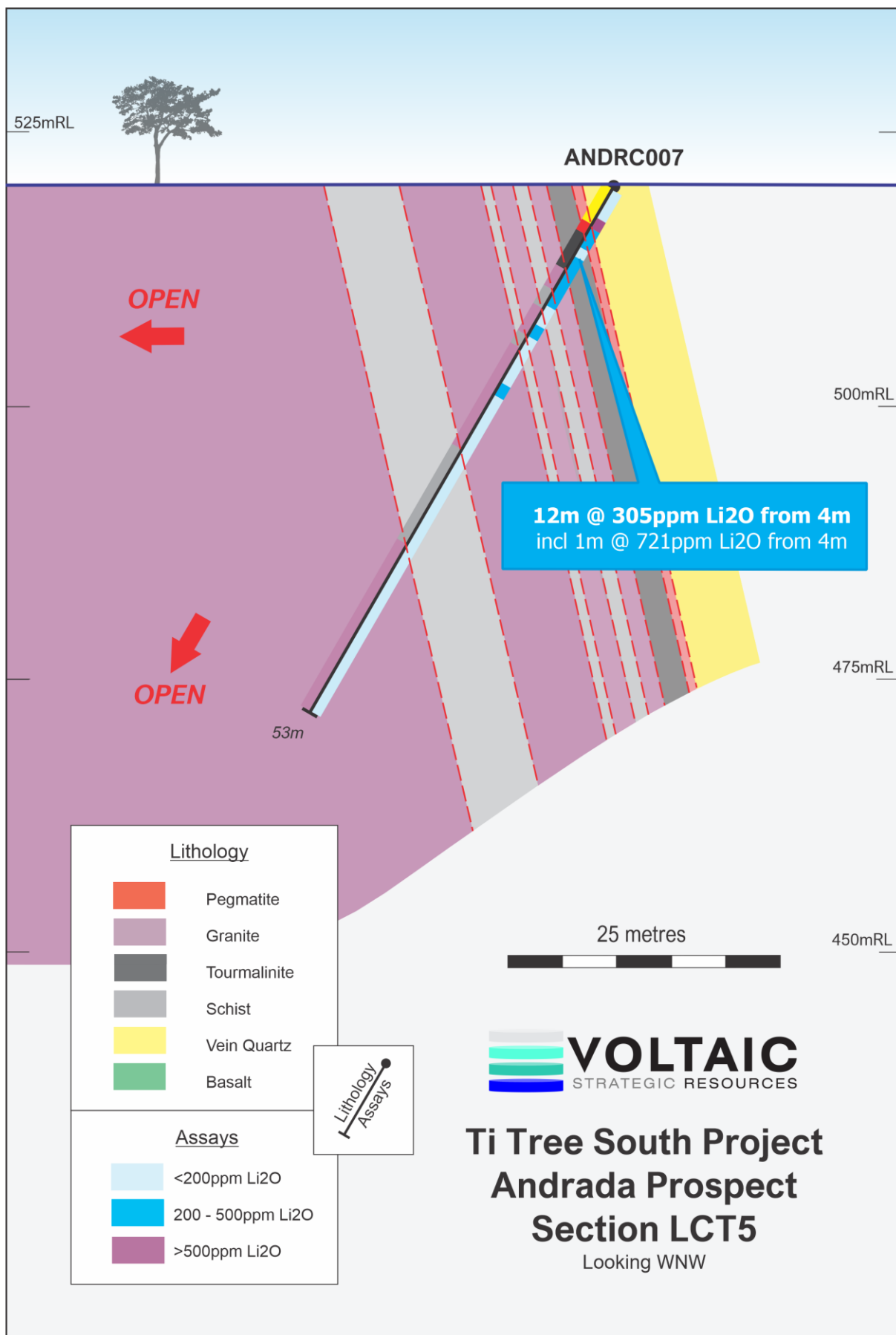
Figure 8. Andrada α Trend: ANDRC007 (LCT5) Cross Section
