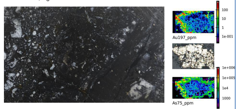
Figure: SHDD506 (256.2m) Mineralised sulphidic jasperoid breccia (10 cm long) Shows Laser Ablation ICP-MS image of a 0.01 mm sulphide grain with high Au-Ag arsenian pyrite/arsenopyrite rim (yellow-red) around low Au-Ag As-poor pyrite core (blue-green).
