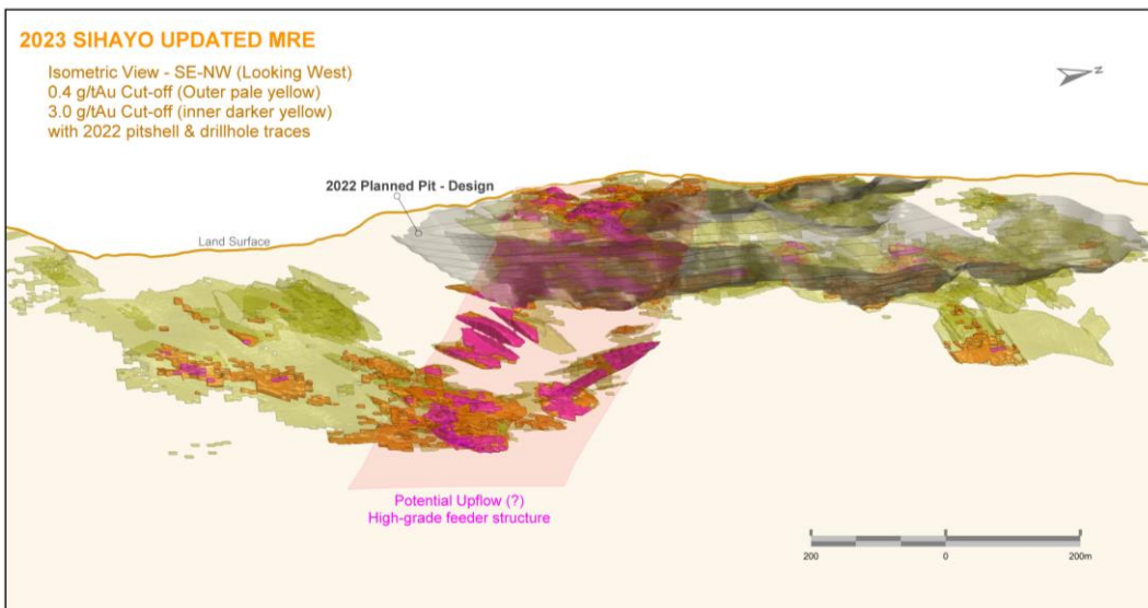
Figure 1: Isometric view of Sihayo gold resource (Looking West)
