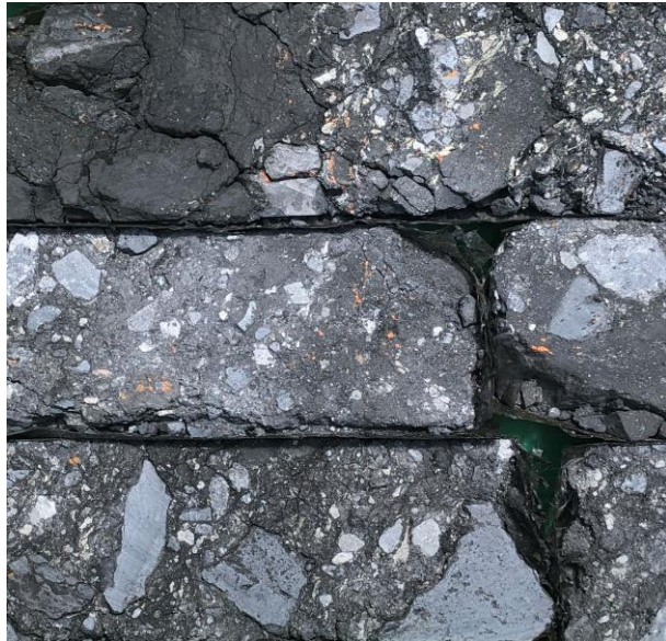
SHDD651: 272.0 – 277.0m Mineralised cave-fill breccia containing jasperoid clasts and fluidized residual clay-sulphide matrix with clots of orpiment Assay Range: 5.69 – 7.68 ppm Au
