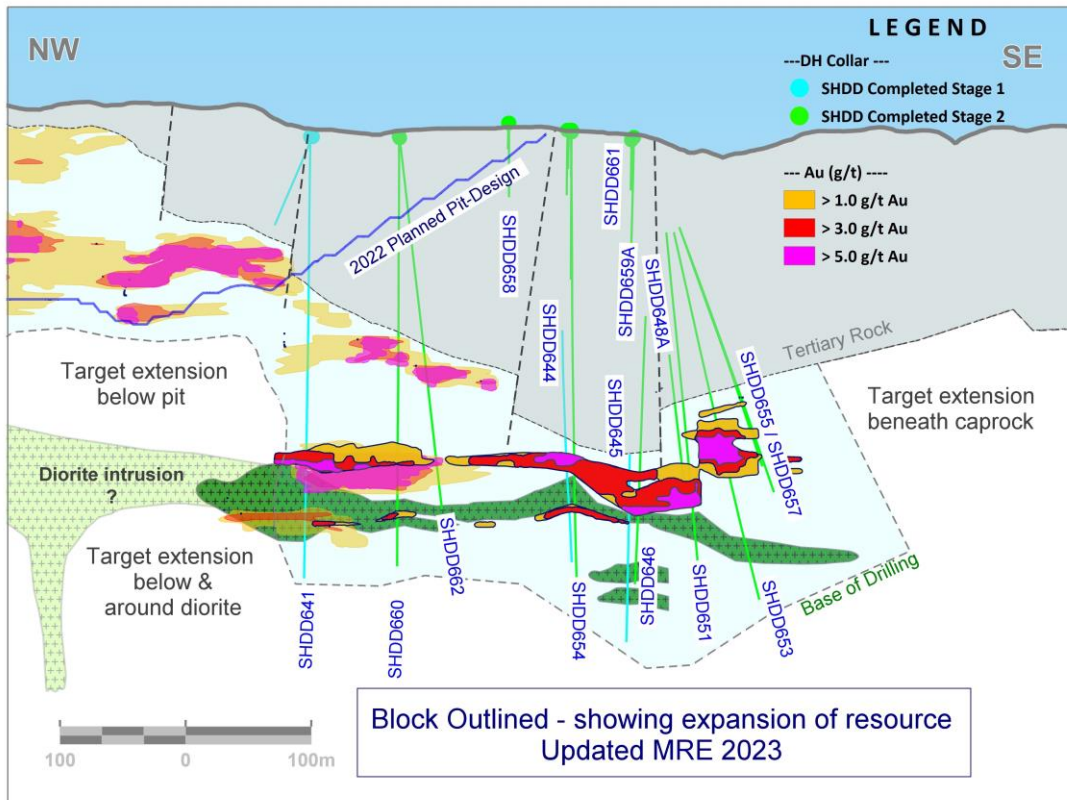
Figure 2: Schematic Long Section of Sihayo underground geology Additional gold resource highlighted bold (within a 25m envelope of section-line)
