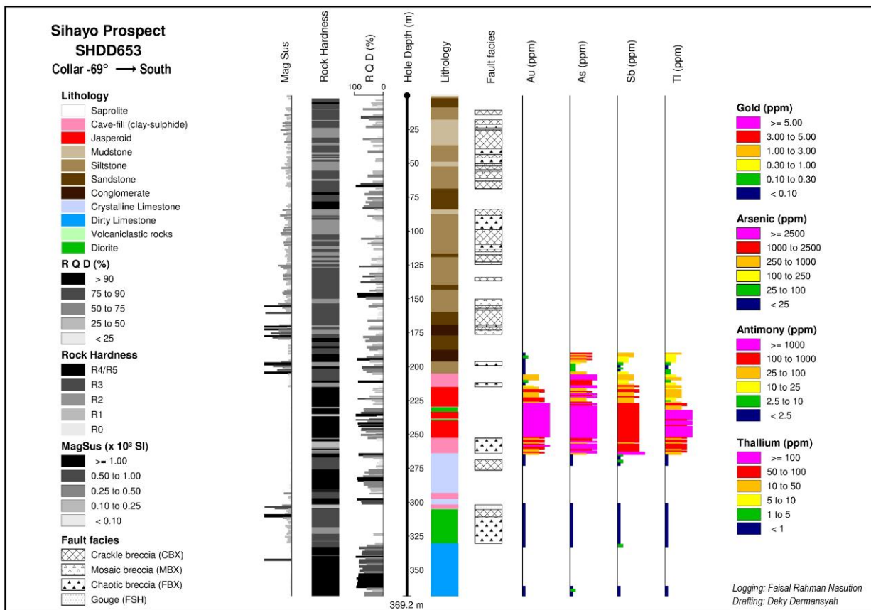
SHDD653 Graphic Summary Log Highlighting the 50m at 7.75 g/t Au intercept in mineralised jasperoid and the strong Au-As-Sb-Tl geochemical association
