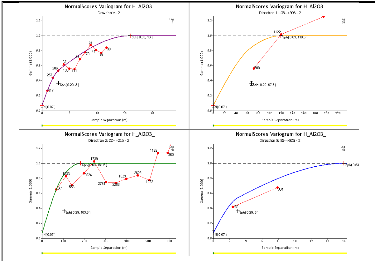
Experimental Variograms Al2O3 (%) for MINDOM 2
