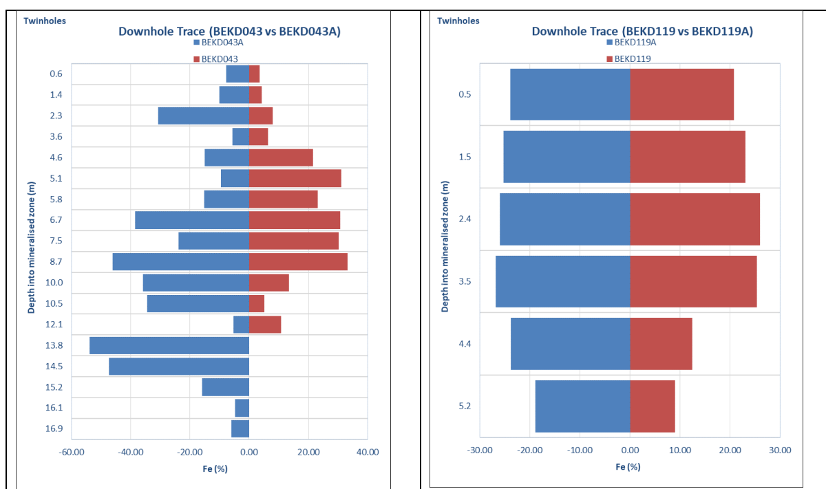
Figure 9.11: Comparison of Downhole Fe Grades for BEKD043 and BEKD043A (left) and BEKD119 and BEKD119A (right)
