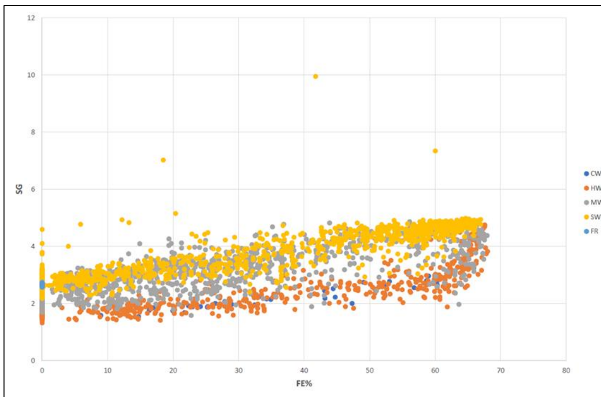
Figure 7.11: Scatter plot Showing Fe Grade Against Density Measurements
