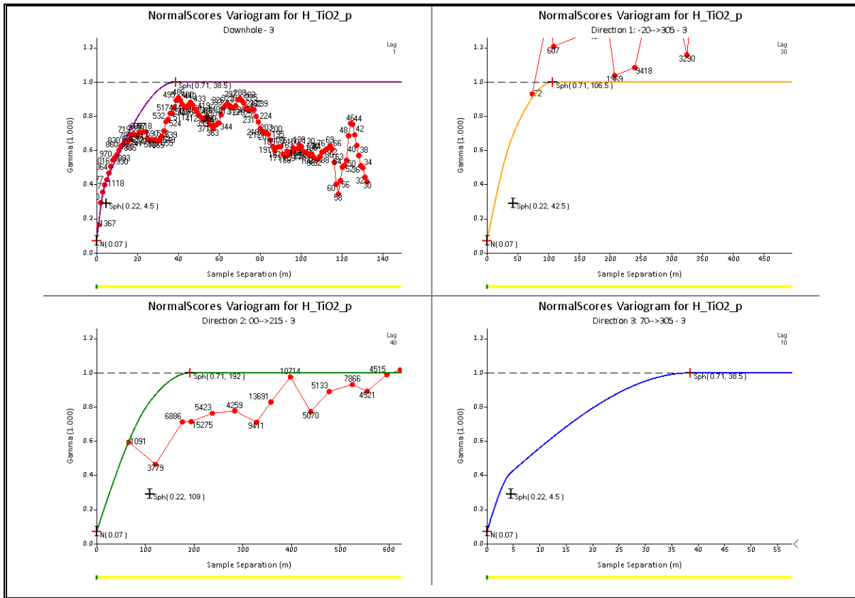
Experimental Variograms TiO 2 (%) for MINDOM 3
