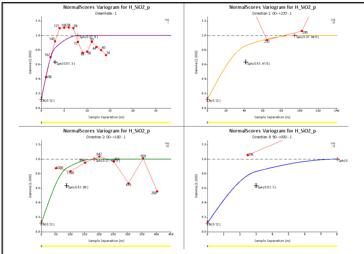
Experimental Variograms SiO2 (%) for MINDOM 1
