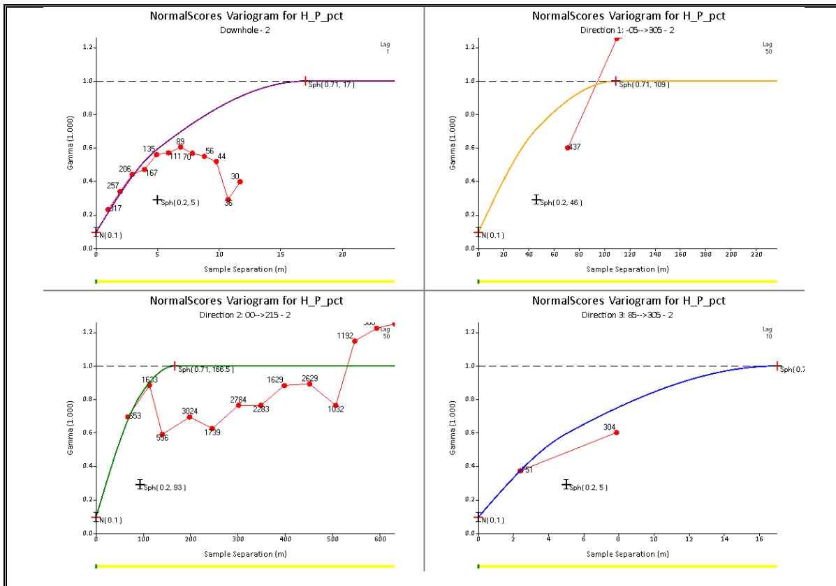
Experimental Variograms P (%) for MINDOM 2
