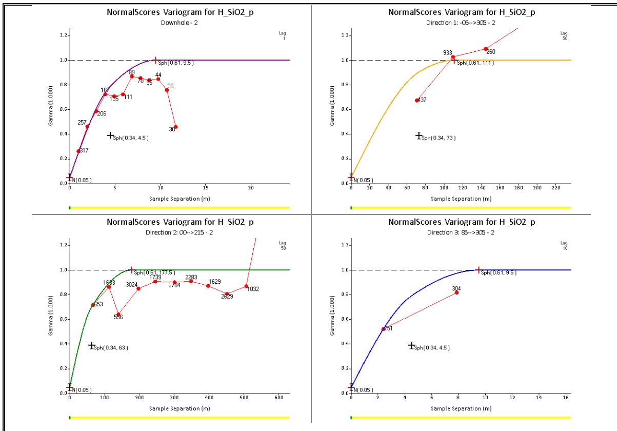
Experimental Variograms SiO2 (%) for MINDOM 2
