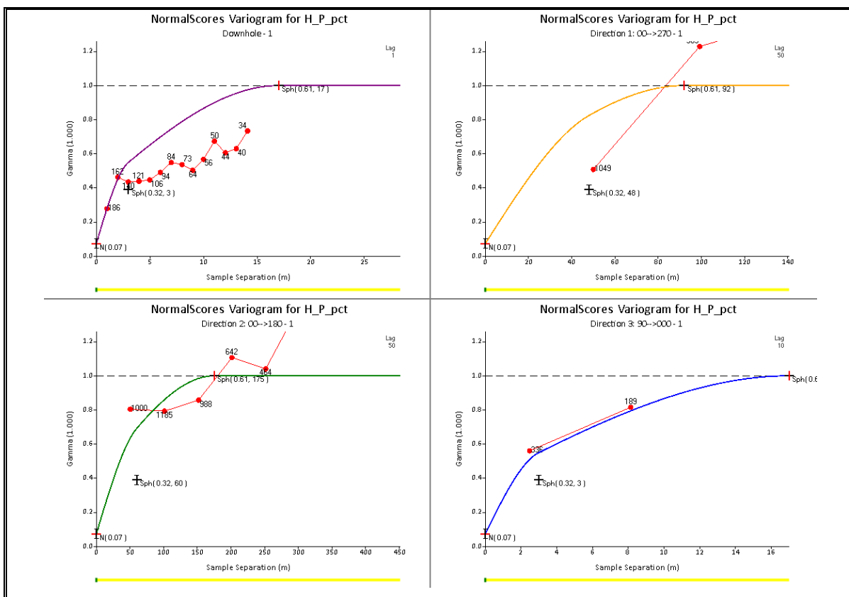
Experimental Variograms P (%) for MINDOM 1
