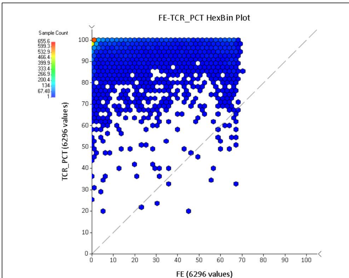
Figure 7.5: HexBin Plot Showing Fe (%) Grades Plotted Against Recovery Values
