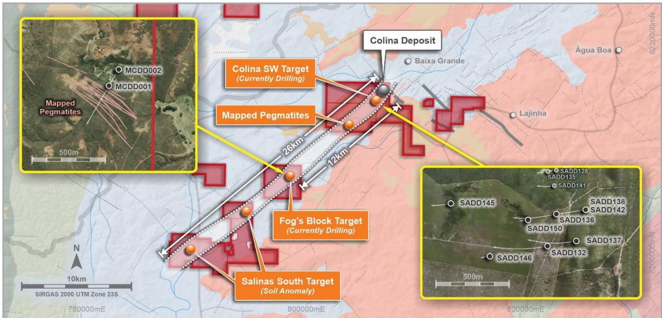
Figure 5: Colina regional drill collar location plan
