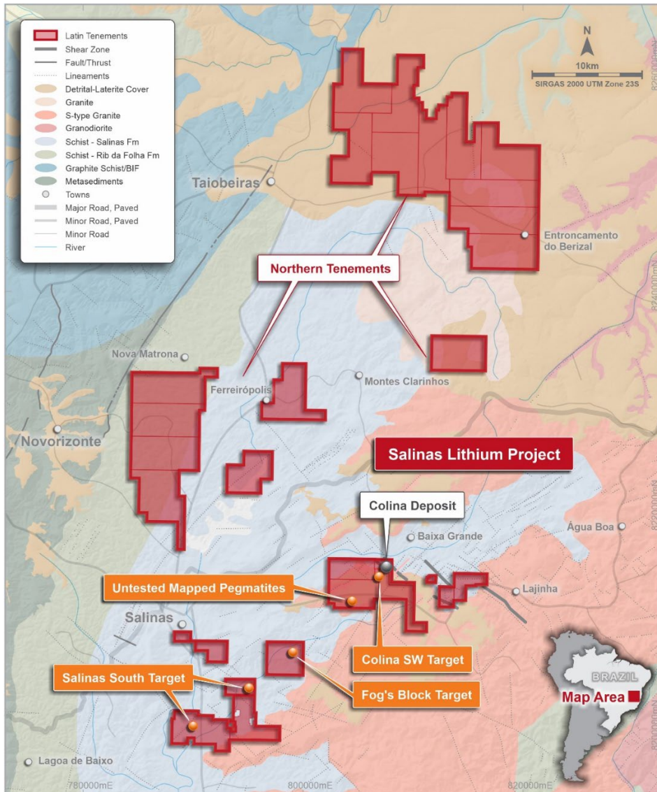
Figure 1: Regional Salinas Lithium Project plan, showing general location of the Colina SW Target, Fog’s Block Target, and Salinas South Target in relation to the Colina Lithium Deposit
