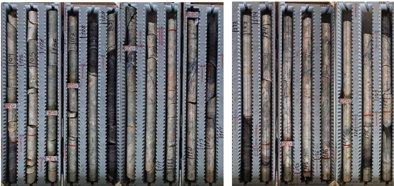
Figure 4: MDCC001- diamond drill core showing spodumene minerals at intervals 103.58 to 107.84m, 108.81 to 113.47m and 172.51 to 179.38m. Refer to Table 2 for further details. The Company draws attention to uncertainty in reporting visual results. Visual estimates of mineral abundance should never be considered a proxy or substitute for laboratory analyses where concentrations or grades are the factor of principal economic interest. Visual estimates also potentially provide no information regarding impurities or deleterious physical properties relevant to valuations. Assay results are expected to be available in approximately 4 weeks.
