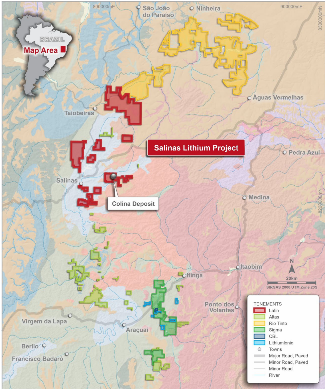
SALINAS LITHIUM PROJECT REGIONAL GEOLOGY AND TENURE
