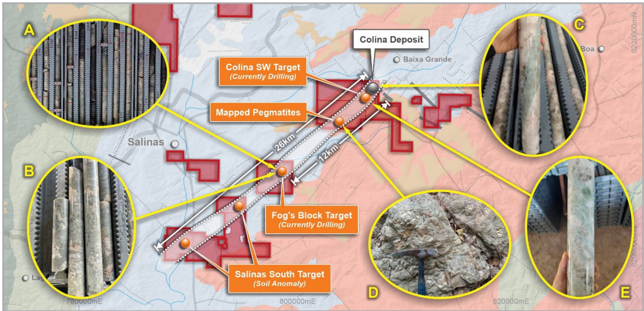
Figure 2: Colina Deposit plan, showing general location and examples of intersected drill core and outcrop samples of the Colina SW Target, Fog's Block Target, and Salinas South Target and untested pegmatite outcrop in relation to the Colina Deposit. A- MCDD001 DD core showing interval 103.35 to 114.69m; B- MCDD001 DD core showing interval 106.95 to 107.54m; C- SADD033 DD core showing interval 321.6 to 322.0m (refer to LRS ASX announcements dated 16 August 2022 and 5 October 2022); D- PMAP251 pegmatite outcrop (804618.11mE, 8211337.703mN); E- SADD132 DD core showing interval 393.53 to 393.83m.
