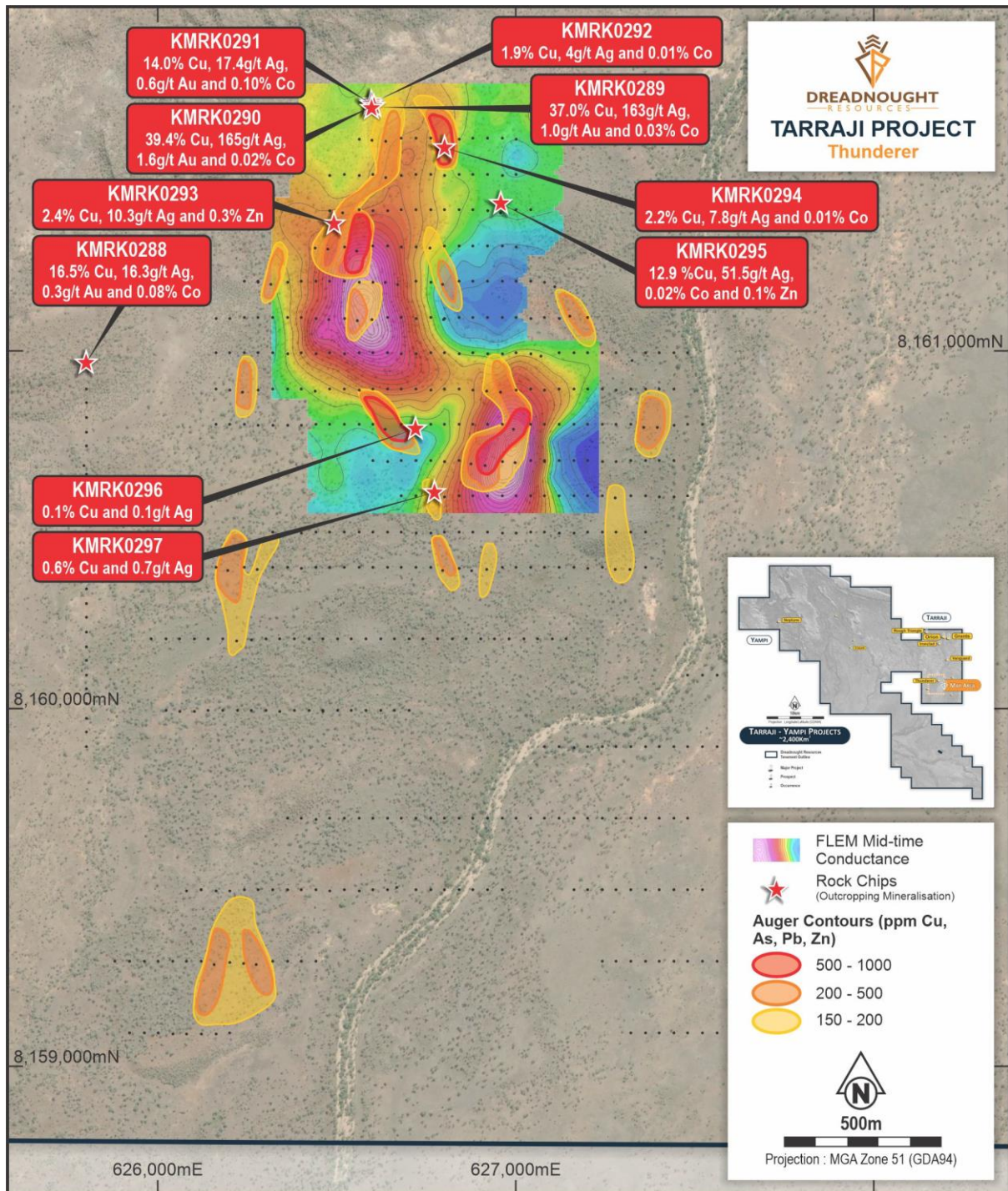
Figure 5: Plan view image of the Thunderer Trend showing the location of prospects in relation to surface geochemical anomaly over a merged mid-time conductance image.
