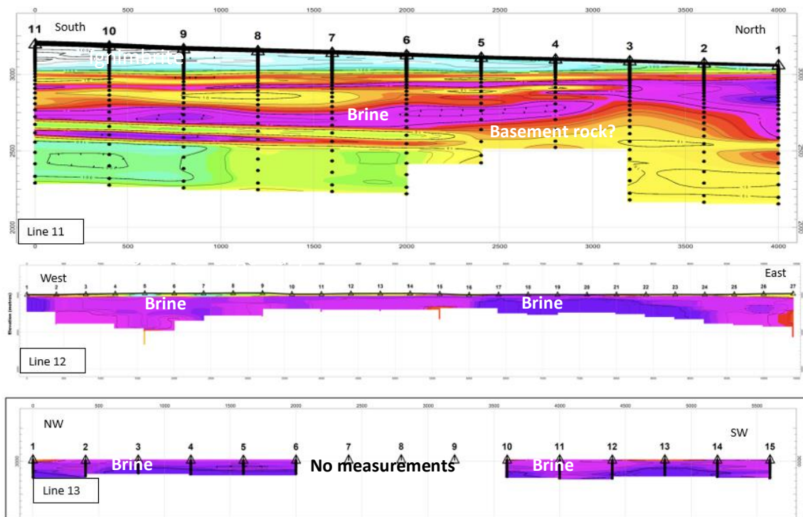
Figure 9: Selected TEM Cross Sections
