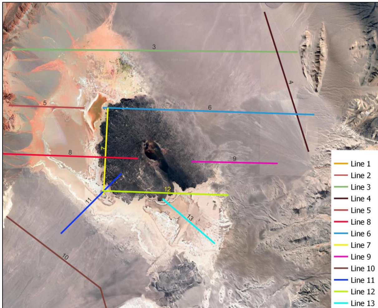
Figure 8: TEM Survey Lines
