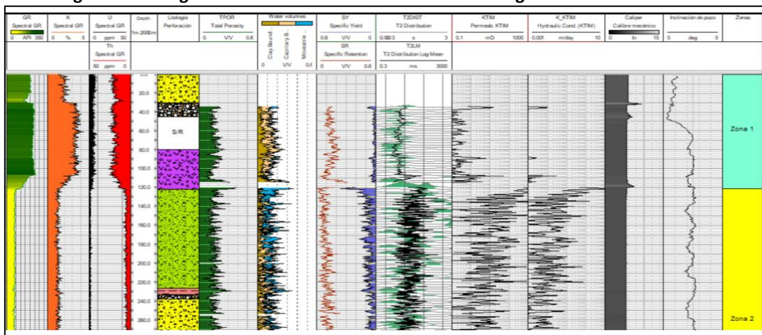
Figure 7: Geophysical log of hole K21D39 showing transition in stratigraphy away from the salar core.
