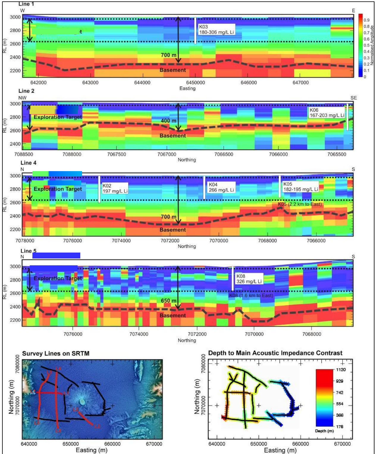
Figure 3: Seismic profiles showing location and depth to basement together with the depths used in the exploration target calculation (red band is the basement reflector)
