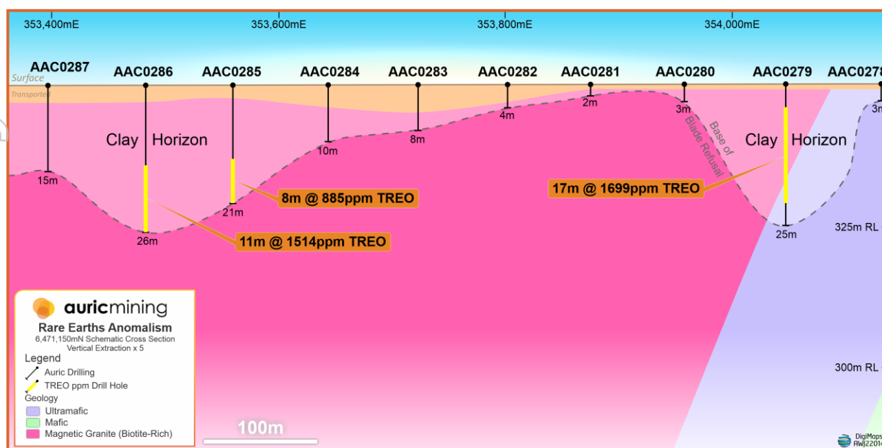
Figure 8. Cross-section of the western part of the drilling line at 6471150N.
