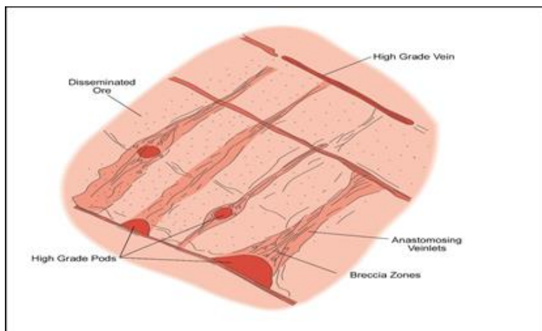
Figure 5: Mineralization at Buena Vista Project
