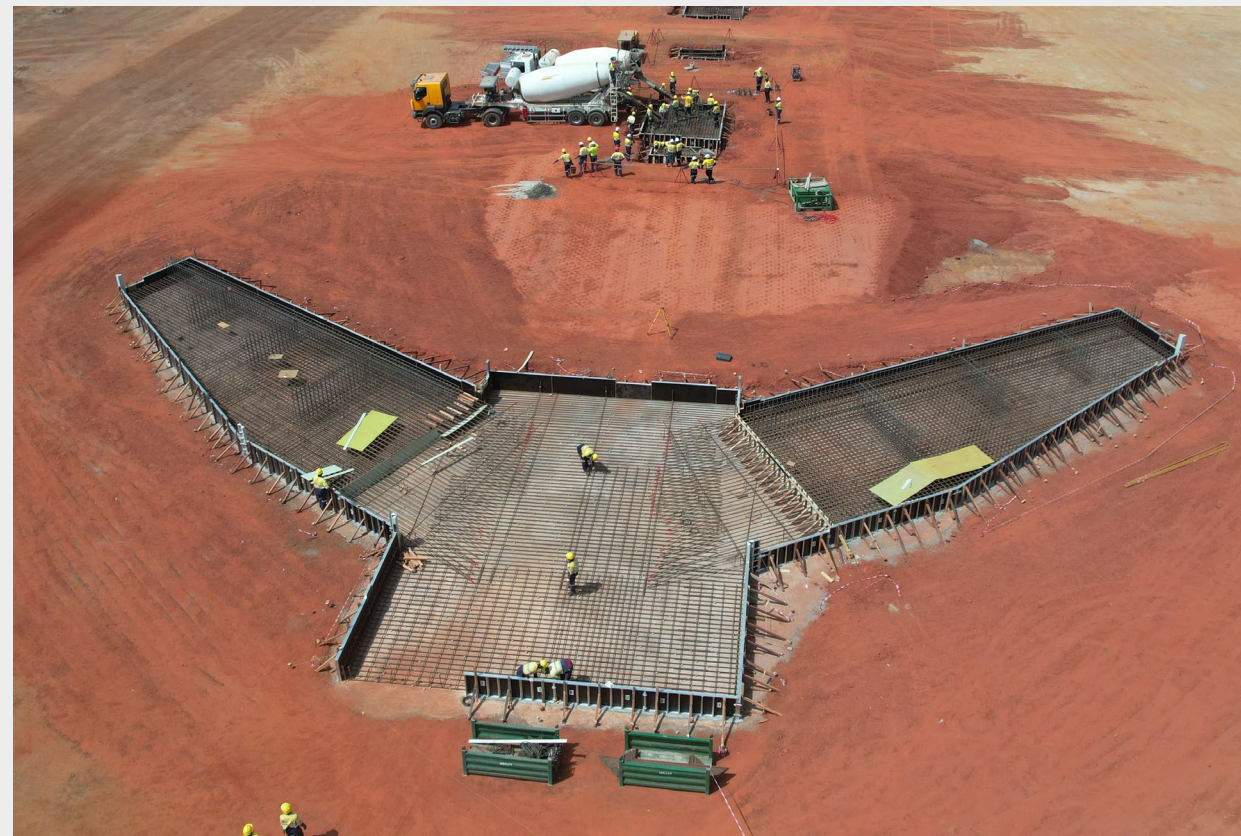
Primary crusher foundations (now poured) & steel installation
