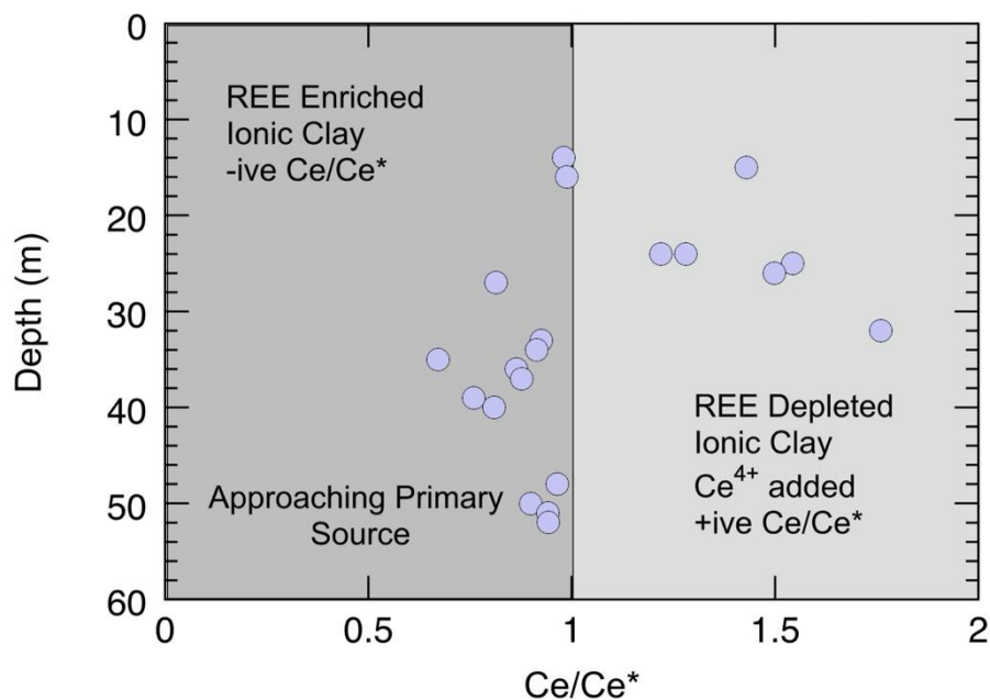
Figure 5. Plot showing variation in Ce/Ce^* with depth in 23NSTRC071. Ce/Ce^* values >>1 indicate that from the surface to approximately 30m Ce^{4+} has developed during weathering (oxidation) of the regolith and has migrated upward in the weathering profile yielding +ive Ce/Ce^* anomalies. By contrast below 30 m the Ce/Ce^* ratios are negative. This is a characteristic feature seen in ionic clay hosted REE systems in China, Brazil, Thailand and Madagascar. The deepest samples in 23NSTRC071 have Ce/Ce^* ratios approaching unity, values typical of primary igneous source lithologies. This plot is interpreted to indicate that between 30 and ~45m the clay (kaolin)-rich regolith sampled in 23NSTRC071, geochemically resembles other ionic clay REE systems.
