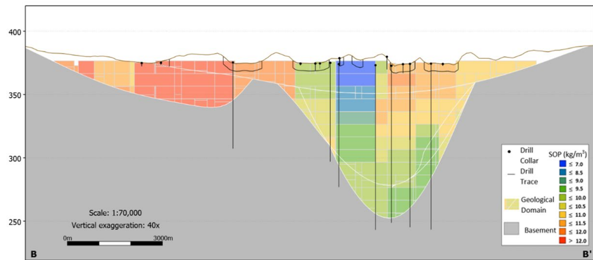
Figure 11: Block model cross section B-B'
