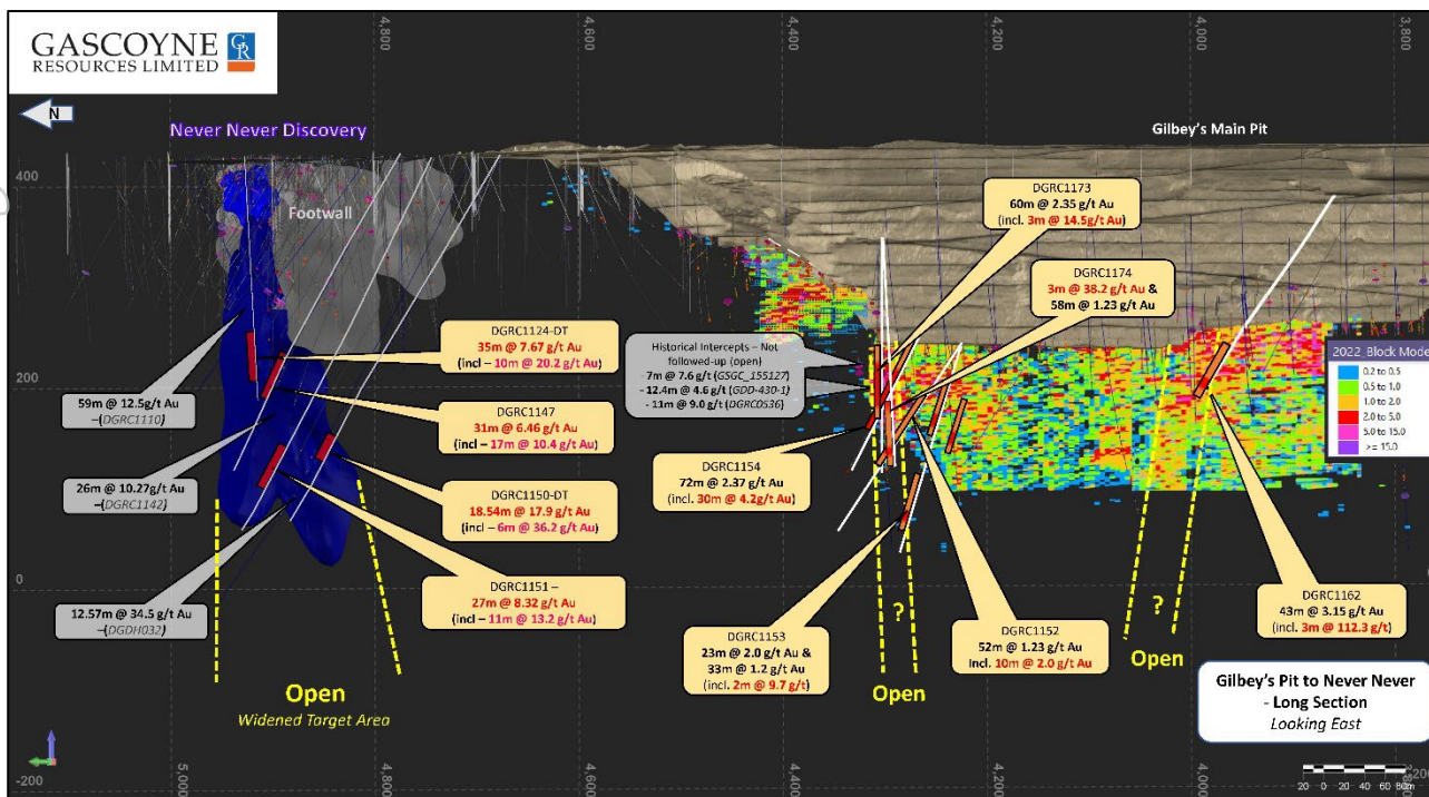
Figure 4: Long-section view looking east through the Gilbey's, Gilbey's North and Never Never Gold Deposits (deposits in order from right to left). Note the yellow "train tracks" illustrate the two main target areas drilled during the initial targeting of Never Never "lookalikes" adjacent to the Gilbey's Pit. The results show elevated grades and widths in both target areas unlike those seen in typical Gilbey's mineralisation and more "Never Never" in orientation (west striking), mineralisation (high silica) and consistently higher grade. Note: the block grades shown beneath Gilbey's Pit represent thick unmined gold mineralisation, open at depth. These areas will be subject to re-estimation during 2023 using more appropriate estimation parameters with an underground mining focus.
