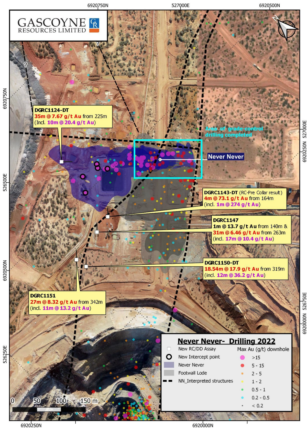
Figure 3: Plan view of east-west Never Never Gold Deposit (dark blue) and north-south Gilbey's North Lode (grey) showing collar locations of results the subject of this announcement.
