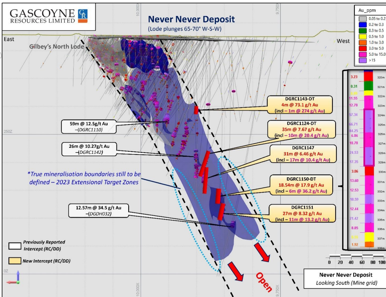
Figure 1: Cross-Section looking south through the Never Never Gold Deposit showing the new resource interpretations and new drill-hole assays being reported in this announcement, with an inset of interval grades from DGR1150-DT on the right side of the image. A number of key previously reported assays are also noted for context. Note: All new assays detailed here are outside the current MRE extents and will be included in the upcoming Never Never MRE update.
