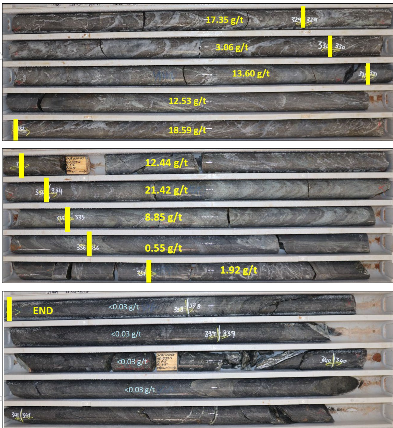
Figure 5: Tray photos of drill-core from DGRC1150-DT (18.54m @ 17.88g/t gold) with overlaid Photon Assay gold grades. Note the heavy silicification and biotite/sericite alteration (pale grey and bronze colouration), with higher grades associated with the more heavily biotitized/sericitized zone (bronze colouration). Strong visual control on mineralisation at Never Never assists greatly in drill design optimisation, interpretation and estimation as well as being invaluable during eventual grade control and mining activities.
