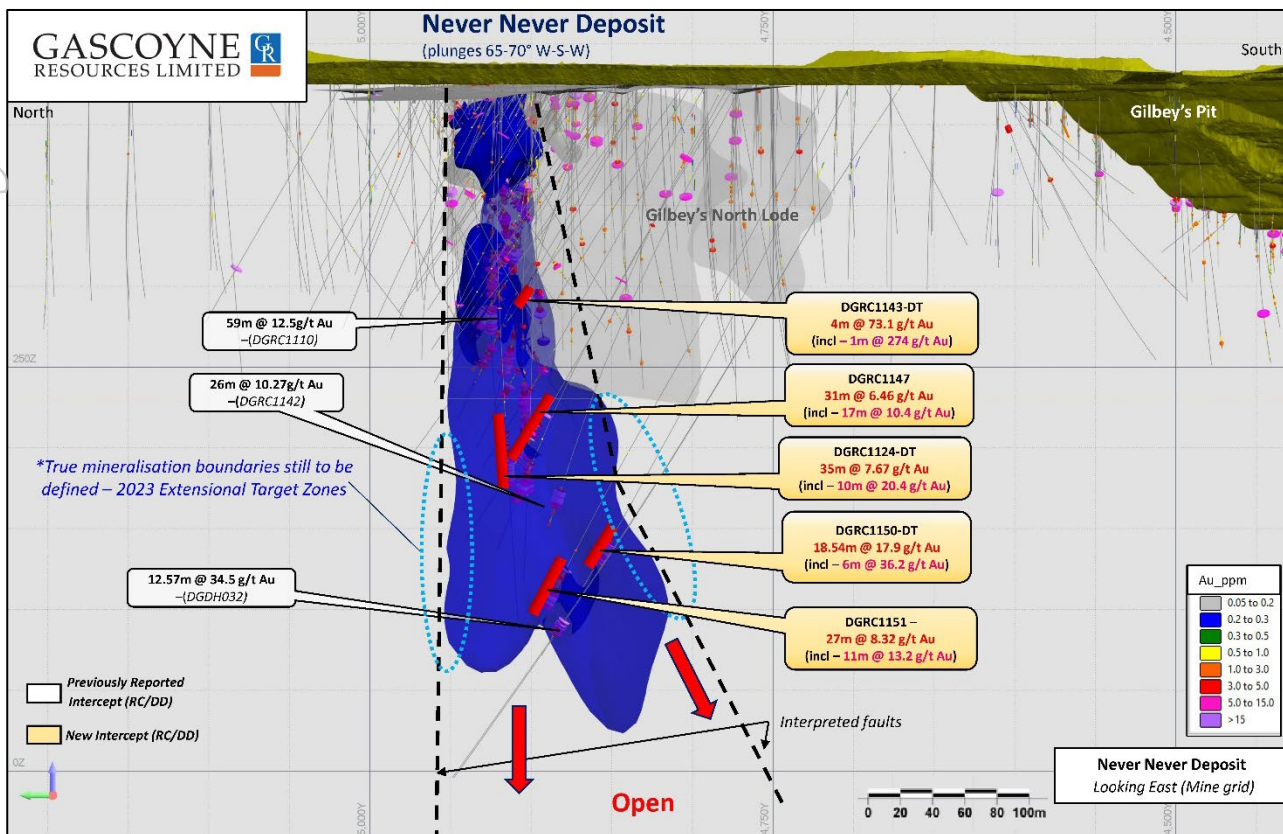
Figure 2: Section view looking east through the Never Never Gold Deposit illustrating recently returned assays showing strong gold mineralisation throughout the central and lower sections of the wireframed interpretation and open down-plunge potential. Note: The Never Never Gold Deposit mineralisation appears to be widening at depth along both the western (Never Never) and southern (Gilbey's) axes.
