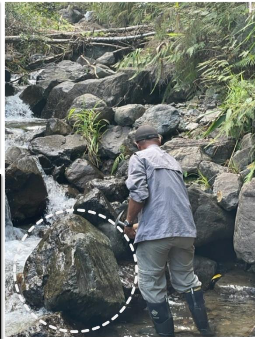
Photo 2: Veri Veri creek float samples include massive nickel sulphide minerals (heazlewoodite, millerite, pentlandite) and nickel-bearing silicates including serpentinite and garnierite. Photo Right: boulder with nickel sulphides in creek. Samples taken by Footprint, see Table 4 and JORC tables in this announcement.
