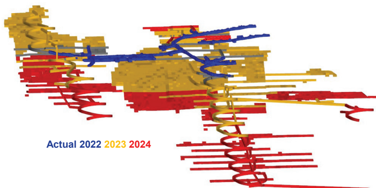
ICO underground mine development plan (October 2022)
