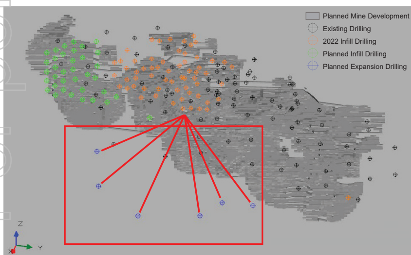
ICO underground drilling plan (October 2022)
