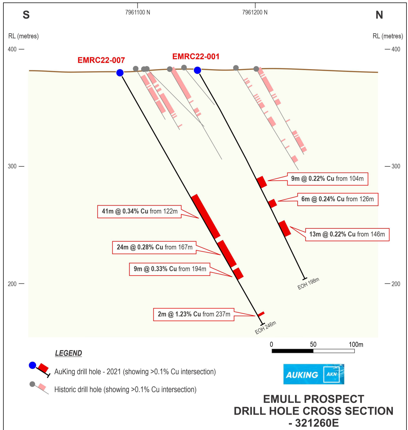
Figure 2. Emull drillhole cross-section plan (holes EMRC22_001 and 007)
