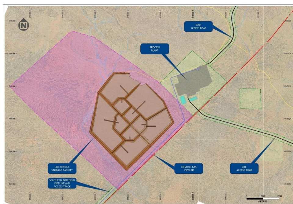
Figure 11: LOM Residue Storage Facility Layout
