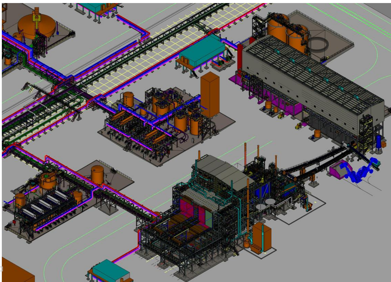
Figure 9: Nolans Hydrometallurgical Plant 3D Model showing the Concentrate Filtration, Pre-Leach, Sulphation Drying, Sulphation and Water Leach Areas
