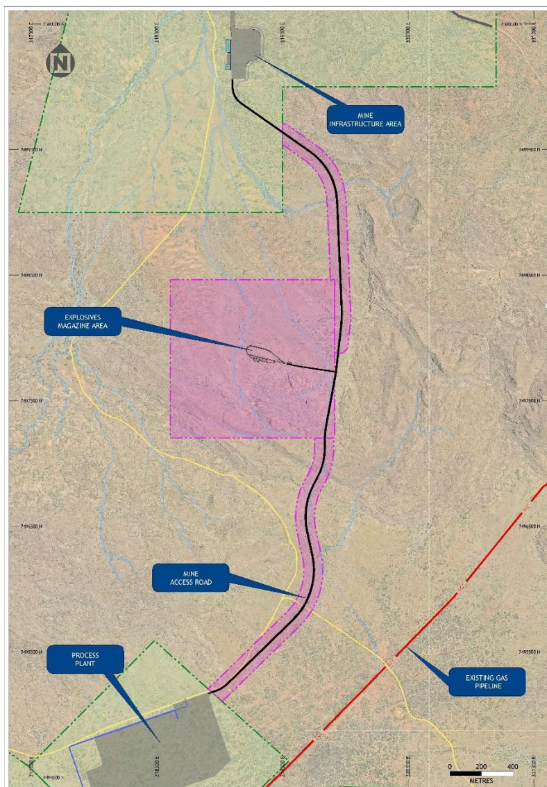
Figure 12: Realigned Mine Access Road and Relocated Explosives Magazine
