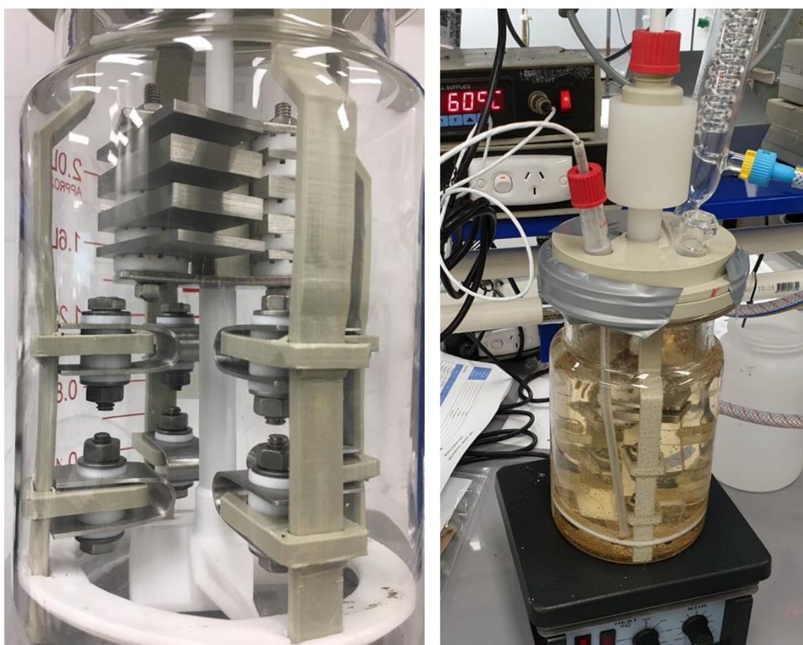
Figure 6: Typical Hydrometallurgical Corrosion Coupon Test Rig and Operation
