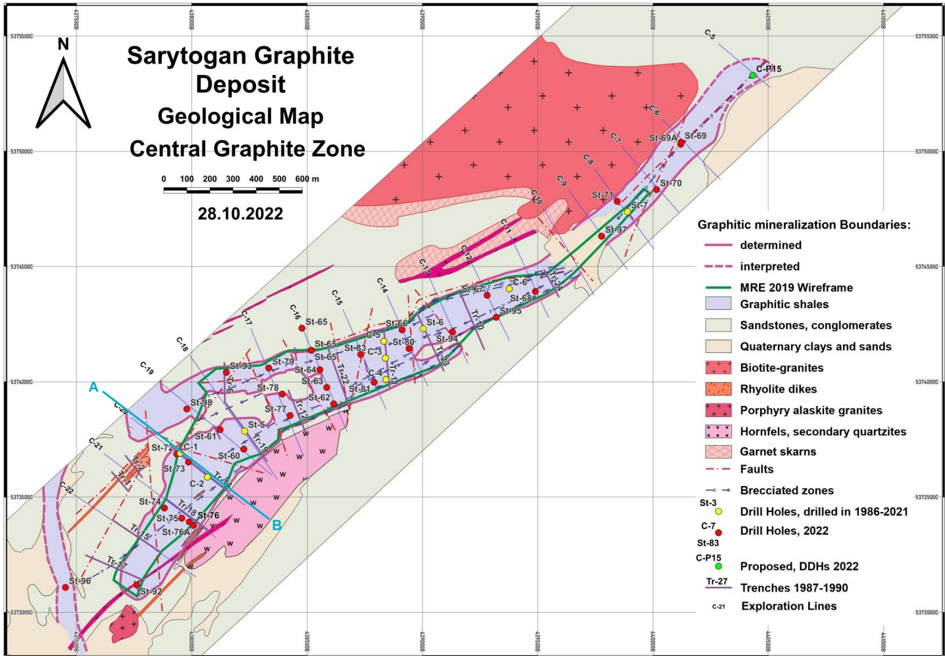
Figure 3 - Completed and Planned Diamond Drilling at the CGZ.
