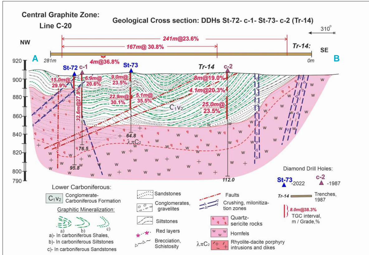
Figure 2 - Geological Cross Section Across Line C-20, Central Graphite Deposit
