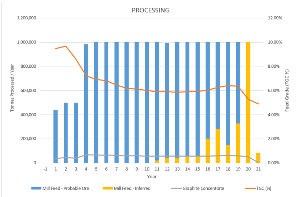
Figure 14: LOM Processing
