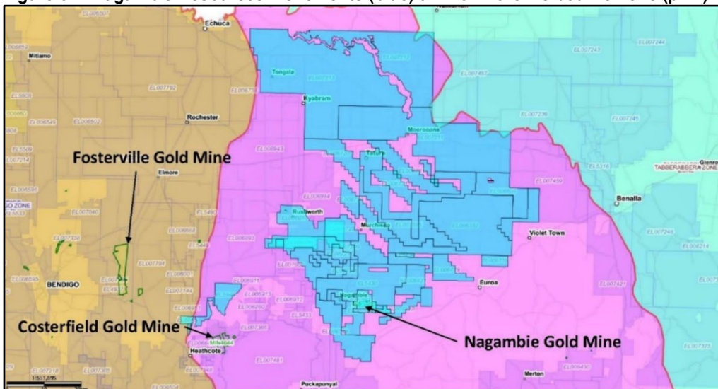
Figure 5 Nagambie Resources' Tenements (blue) all within the Melbourne Zone (pink)
