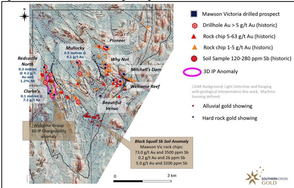
Figure 4 Plan of Redcastle showing Geological Detail
