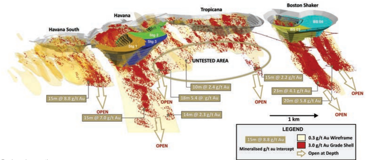
Tropicana long section.
