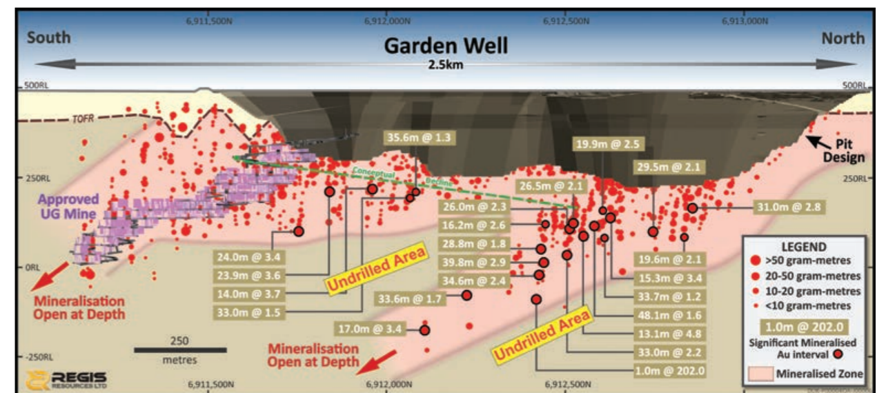
Garden Well long section looking west showing high grade intersections under Main pit, and the existing underground mine design at Garden Well South.
