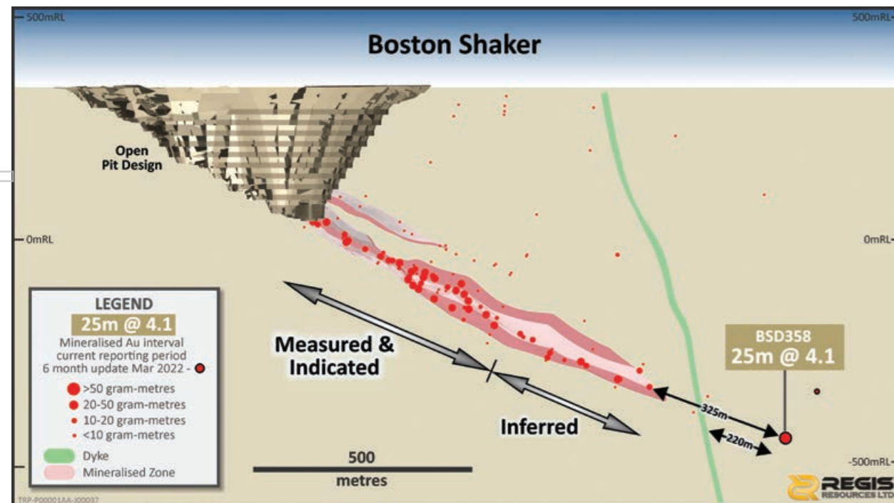
Boston Shaker Cross-section A-A showing the down-plunge continuation of economic mineralisation down plunge outside of the current modelled mineralised zone.
