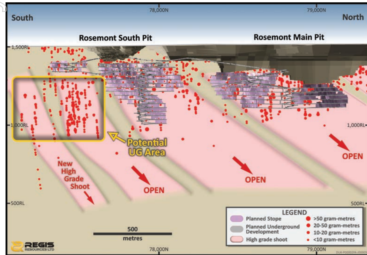
Rosemont South long section showing high grade intersections
