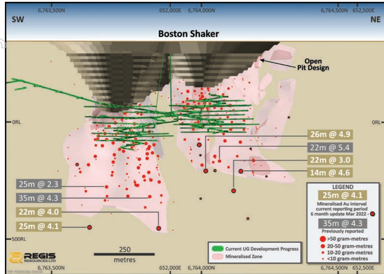
Boston Shaker long-section displaying gram metre pierce points and 0.3g/t Au mineralisation zone and recent high grade intercepts outside of the current modelled mineralised zone.
