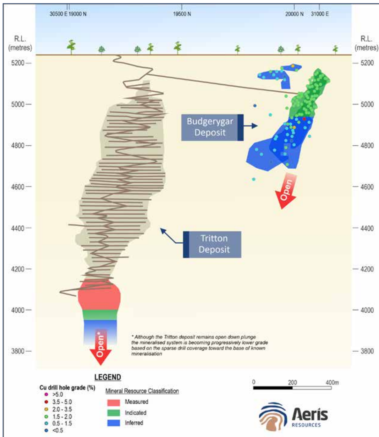
Budgerygar Underground Mine section
