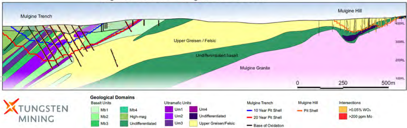
Figure 5: Interpreted geological domains (and sub-domains) at Mt Mulgine. Possible relationship / connectivity between the Mulgine Trench and Mulgine Hill deposits has been clarified for the first time.
