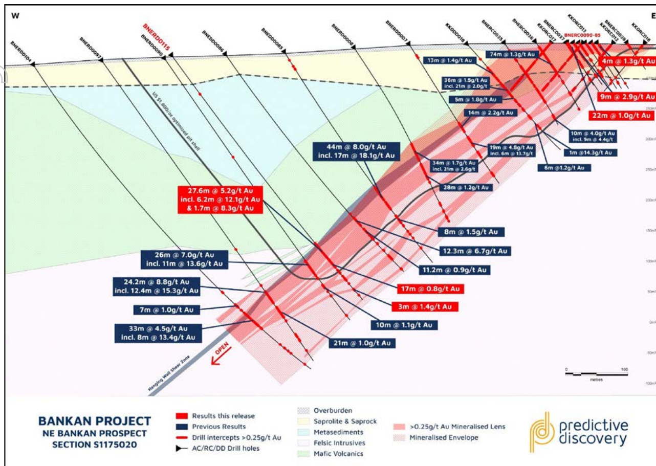
Figure 10 - Section 1175020N (+20mN/- 40mS) with holes BNERD0115.
