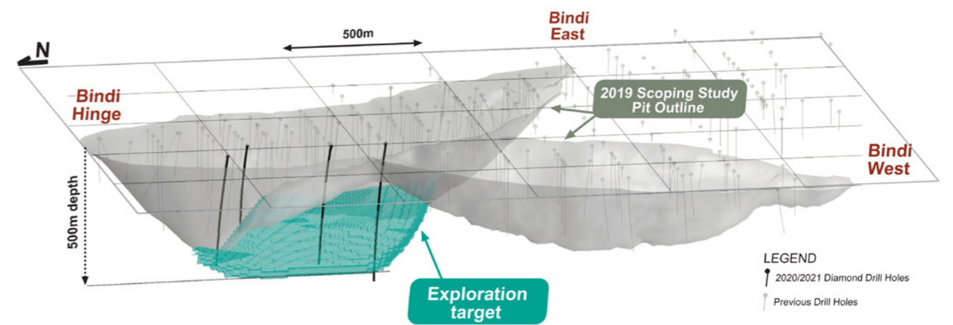
Figure 4: Oblique 3D view of the Bindi Deposit showing 2019 Scoping Study open pit shells and location of the Exploration Target. Highlighted are the deep diamond drill holes on which the Exploration Target is based.
