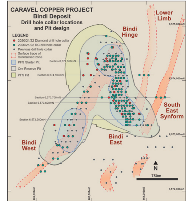
Figure 3: Bindi deposit drill hole collar locations and pit design
