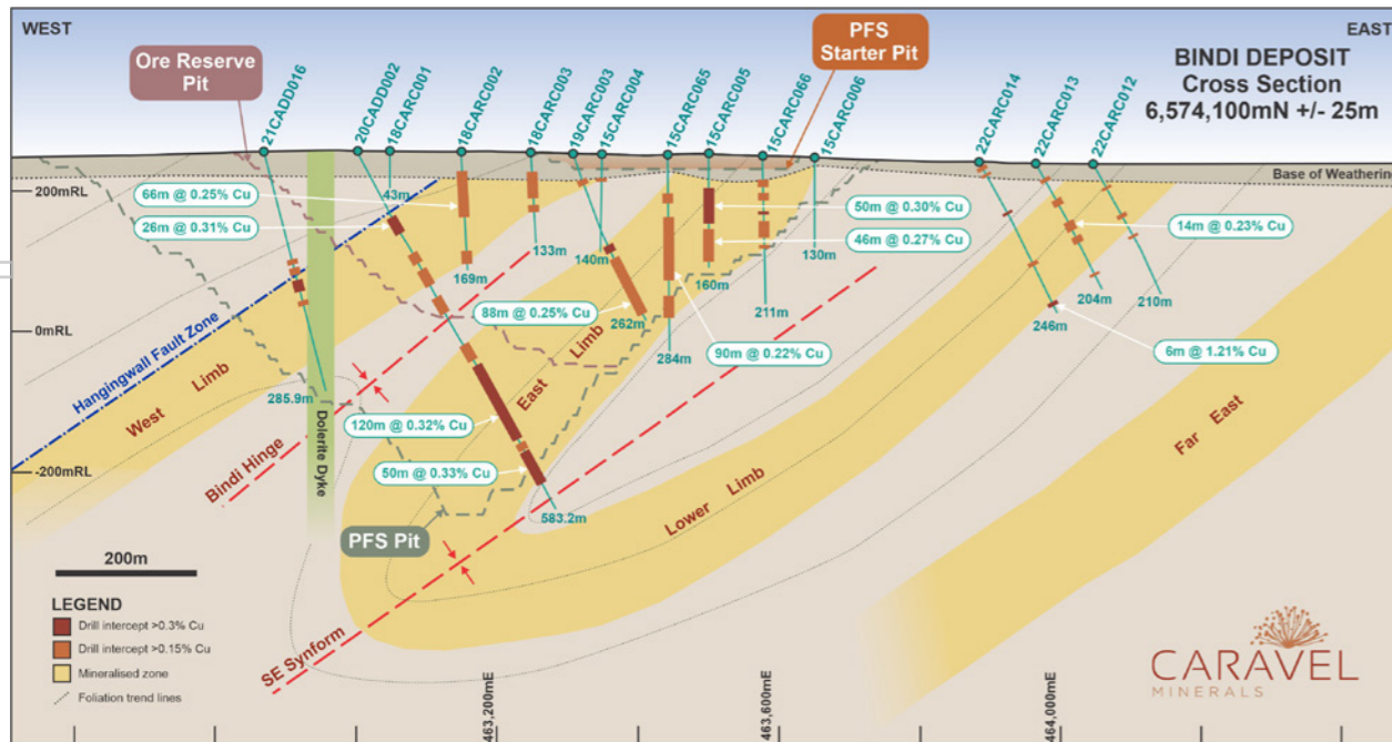
Figure 1: Bindi South East Synform Cross Section Showing Lower Limb and Far East Positions
