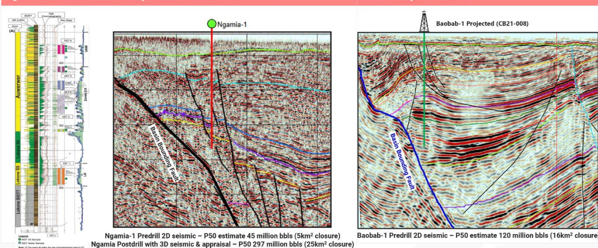
Figure 2 - Ngamia-1 vs. Baobab-1 pre-drill seismic cross section comparison
