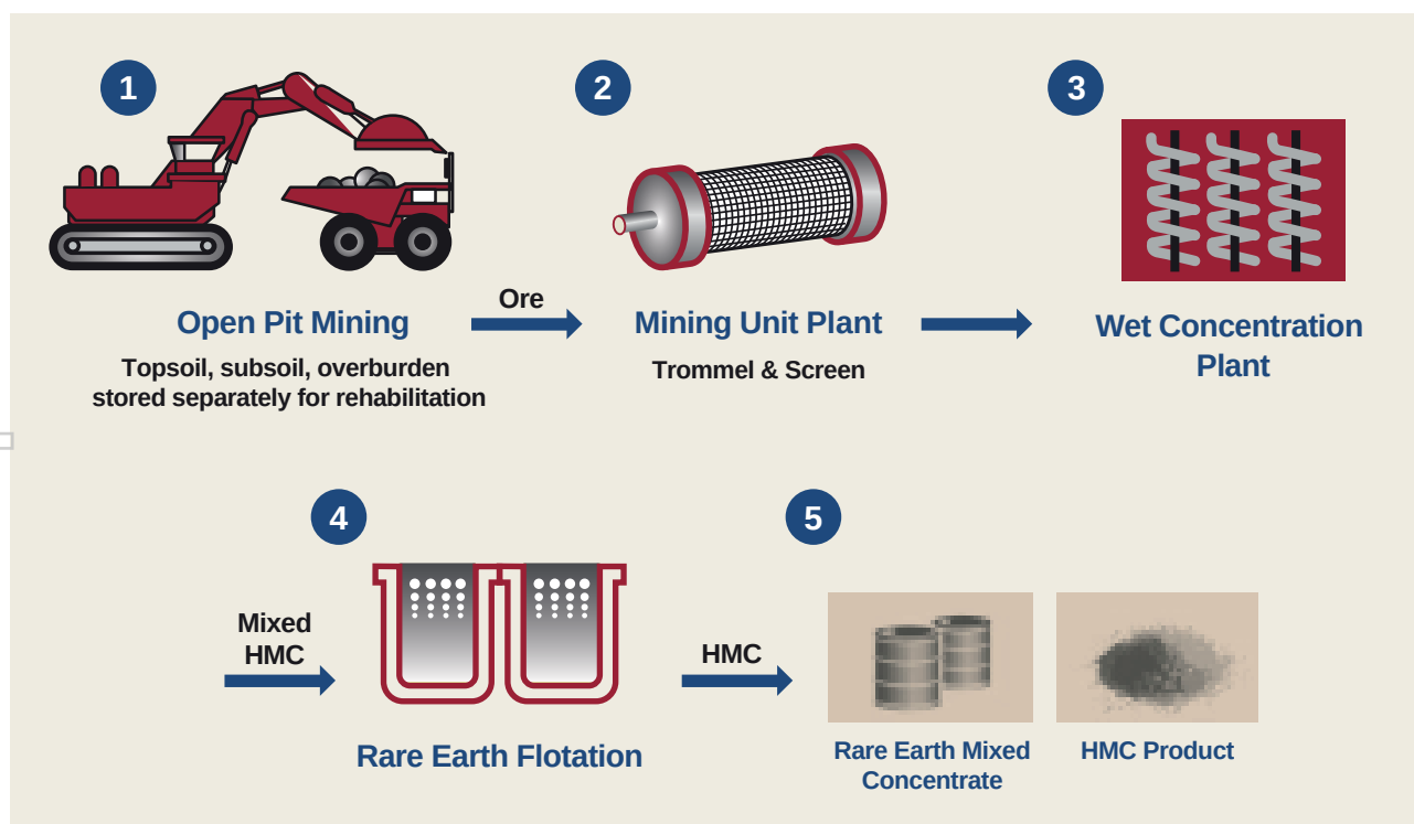
Donald Project Simplified Phase 1 Process Flow-Diagram
