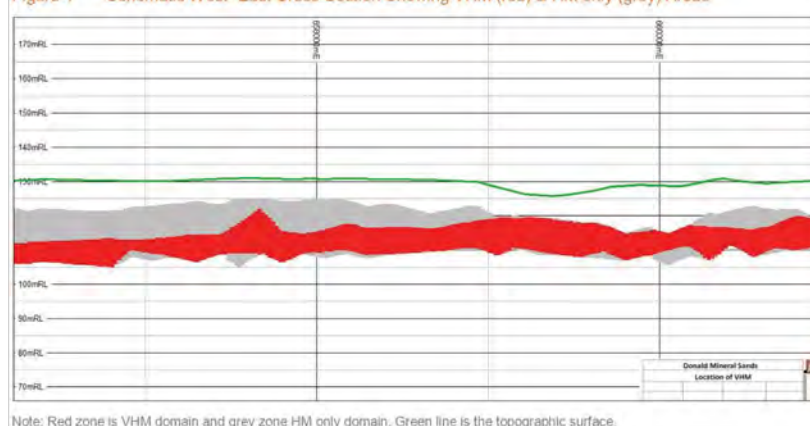
Figure 1 Schematic West- East Cross-Section Showing VHM (red) & HM only (grey) Areas
