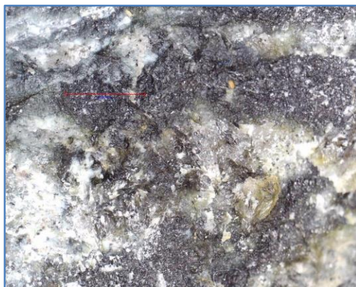
Figure 11: Quartz-biotite altered mafic in 22WAC0030, 49-50m (red bar 5mm)
