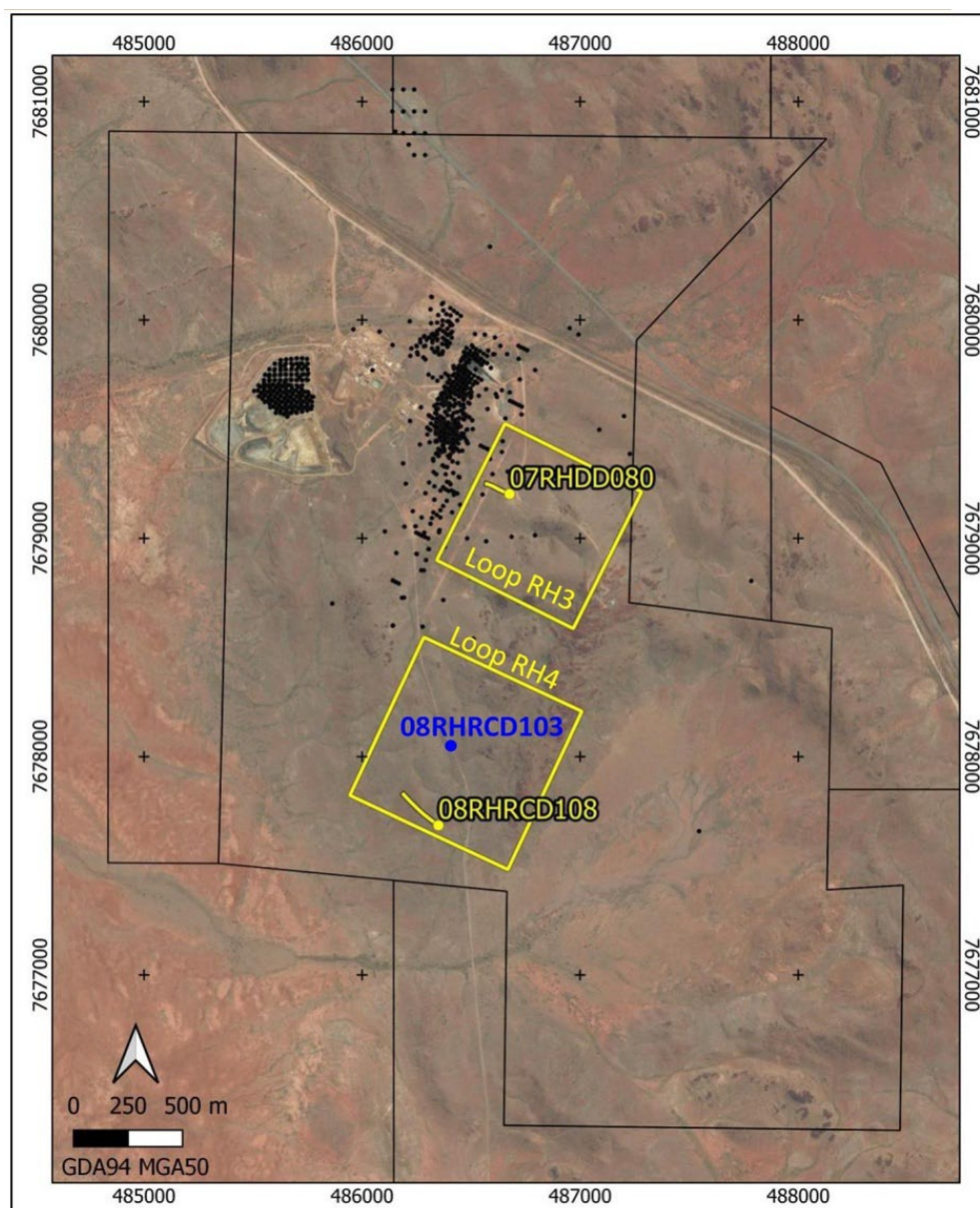
Figure 40: Downhole electromagnetic survey loops and drill hole locations that underwent the survey.
