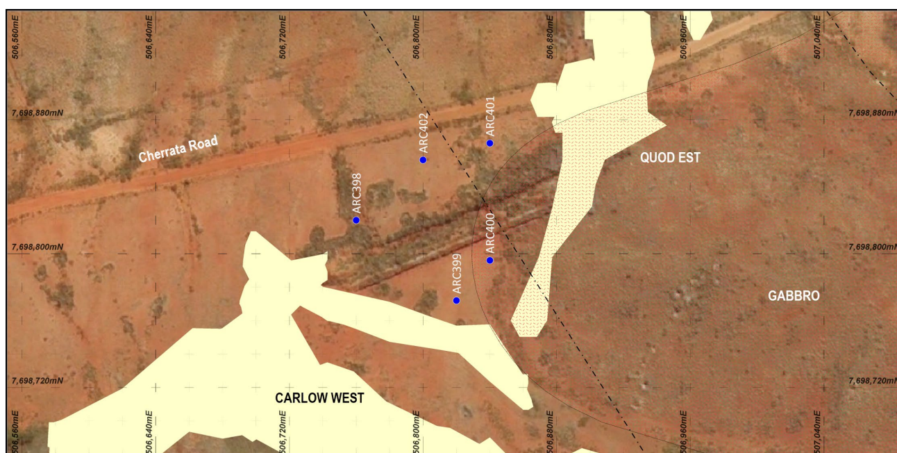
Figure 26: Location of Carlow West drill holes. Note trend of a NW structure in the vicinity of ARC401. Yellow solids are Carlow mineralised polygons.
