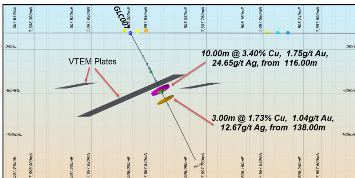
Figure 32: Slight oblique section looking northeast along the drill trace of GLC007 showing the location of the high-grade intersections in relation to the VTEM plates.
