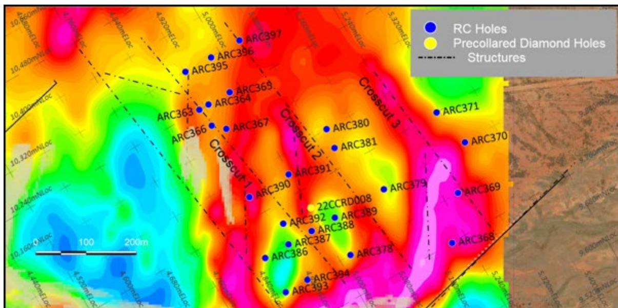
Figure 18: Drill collar location on background of SAM survey. Note the strong to intense SAM anomaly to the east which has defined conductive ultramafic rocks.
