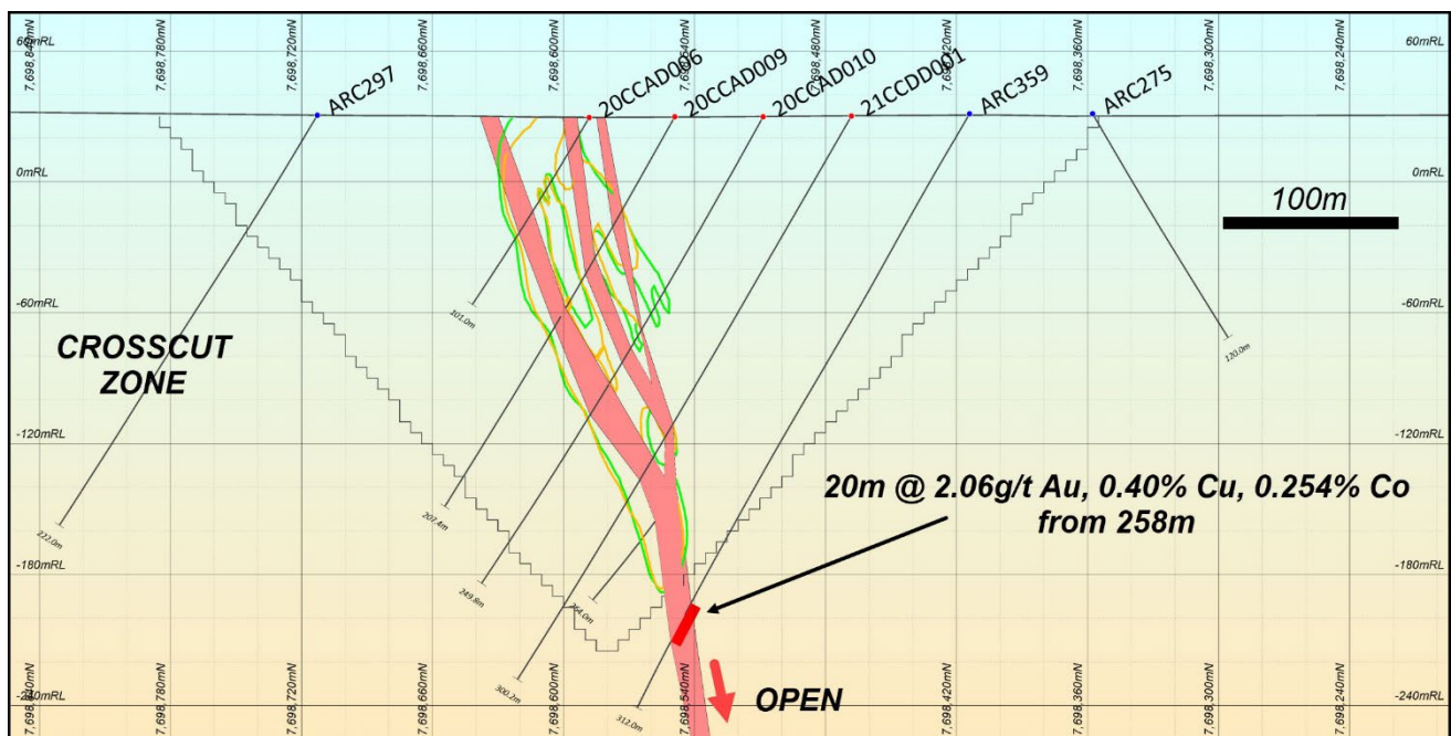
Figure 22: Hole ARC359 Section 507540mE highlighting the thick mineralised intersection outside of the 2021 optimised pit outline. This mineralised trend remains open down dip. The line traces highlight the low grade halo with orange outlining the >0.25g/t Au trace and green outlining >0.25% Cu as defined by implicit modelling. Refer to Figure 11 for location of the section.
