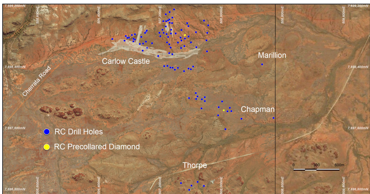
Figure 8: Location of drill collars in the various prospects within the Carlow tenement E47/1797.
