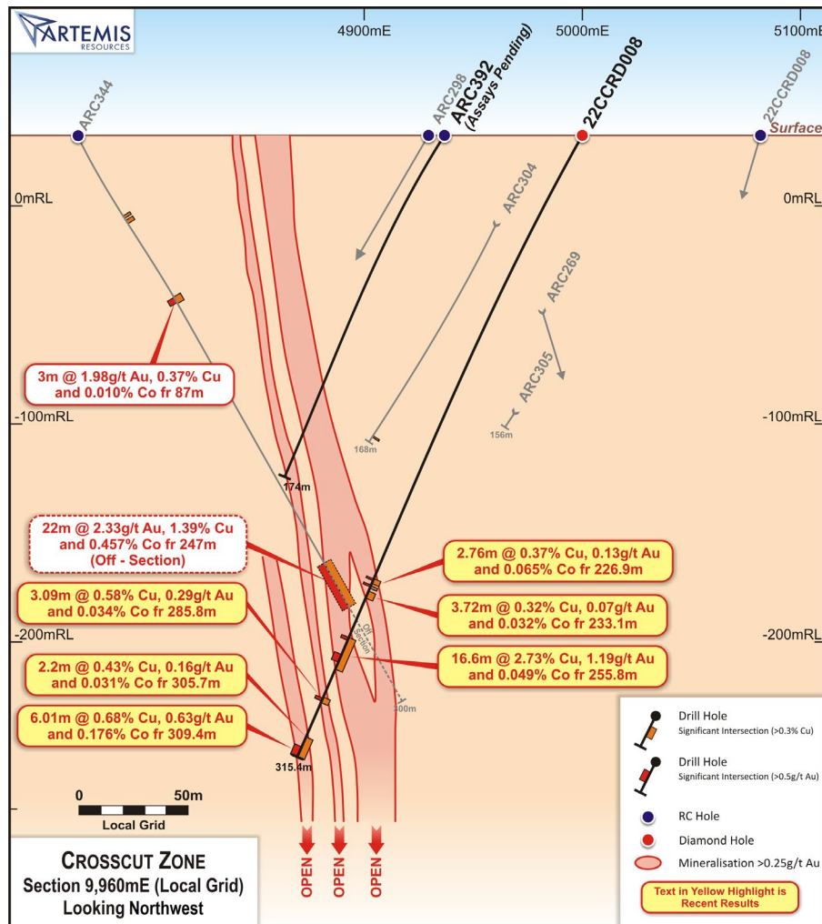
Figure 10: Section 9,960mE showing significant intersections for hole 22CCRD008. High grade intersections for ARC344 included for comparisons. Hole ARC392 drilled updip from the massive sulphide occurrence is pending assay results. Refer to Figure 8 for section location.
