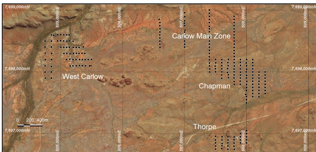
Figure 38: Overview map showing the distribution of UFF soil sampling that cover the Carlow Castle, Chapman and Thorpe (Little Fortune) areas.
