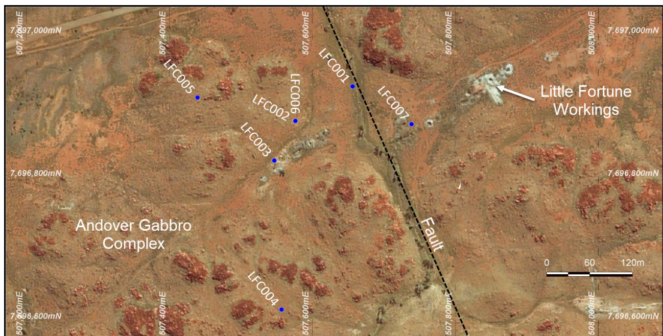
Figure 34: Diagram showing collar locations and simply geology for the Little Fortune Prospect.
