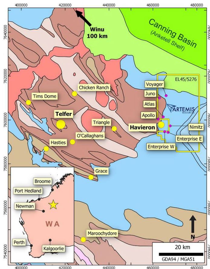
Figure 2: Paterson Central Tenement E45/5276 (yellow outline) overlying main geological units, and showing locations of major gold and base metal deposits. Green; Anketell Sediments, Blue; Paterson Formation, Dark Brown
