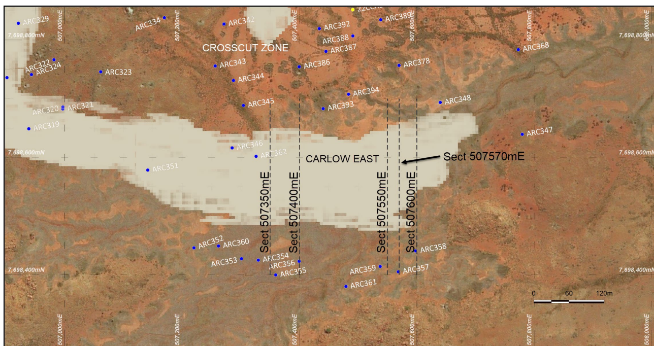
Figure 19: Section lines and collar locations of holes for the East Zone.
