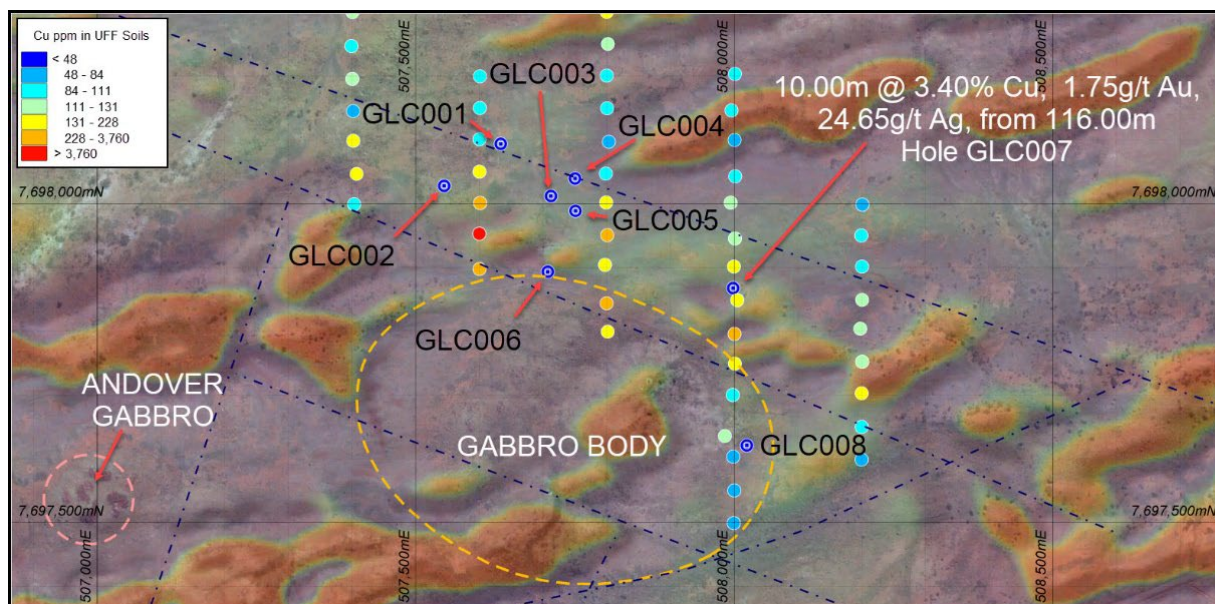
Figure 33: Image showing the first pass UFF soil sampling for Cu values, which are highlighting a NW trend. Note that the significant Cu values occur within the two inferred bounding structures, also trending to the NW. Hole GLC007 is highlighted with its significant result, using a 0.3% Cu cut off. Image is mag 2VD with draped satellite image.
