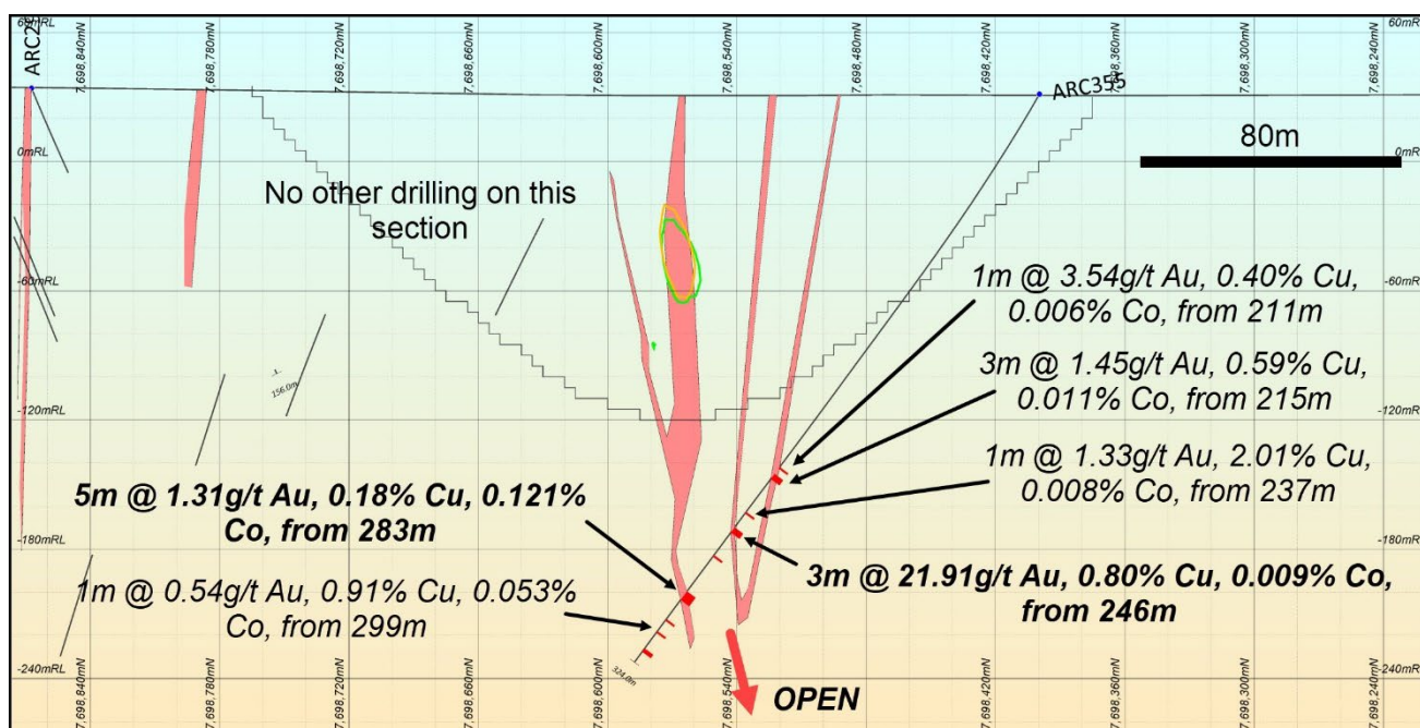
Figure 20: Hole ARC355 Section 507360 showing a series of mineralised intervals down along the drill trace, well below the 2021 optimised pit outline. This remains open at depth. The line traces highlight the low grade halo with orange outlining the >0.25g/t Au trace and green outlining >0.25% Cu as defined by implicit modelling. Refer to Figure 11 for location of the section.
