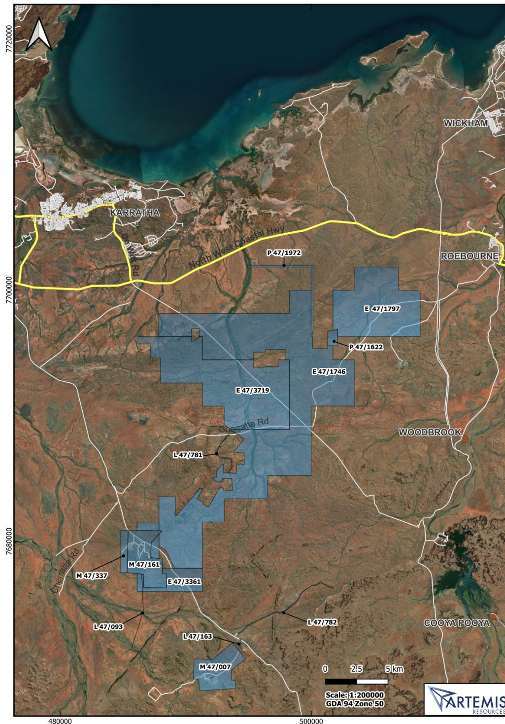
Figure 7: West Pilbara project map highlighting Artemis' current tenement holdings.
