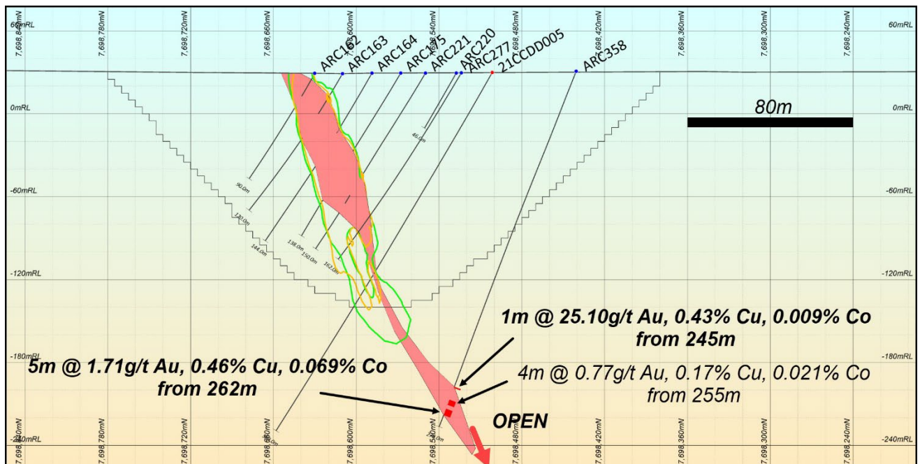
Figure 24: Hole ARC358 Section 507600mE showing the continuation of the mineralisation at depth and well below the 2021 optimised pit outline. The line traces highlight the low grade halo with orange outlining the >0.25\text{g/t Au} trace and green outlining >0.25\% Cu as defined by implicit modelling. Refer to Figure 11 for location of the section.
