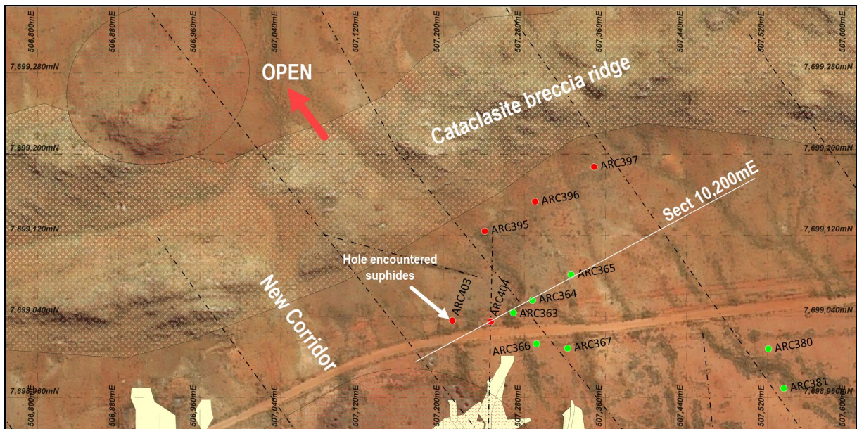
Figure 15: Showing the location of the holes to test the mineralisation to the north. ARC403 encountered sulphides but assays are pending. Interpretation of the magnetics have identified similar NW structures to the west and NW along strike. These are north of the cataclasite ridge which is considered prospective for mineralisation.
