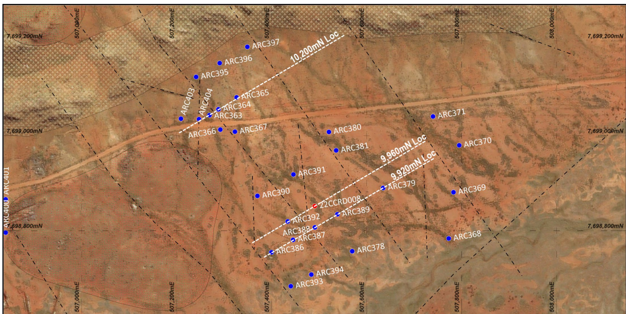
Figure 9: Location of drill holes at Crosscut and section lines. Note that only holes ARC403 and ARC404 were completed during the quarter period. Other holes are referenced in section figures.
