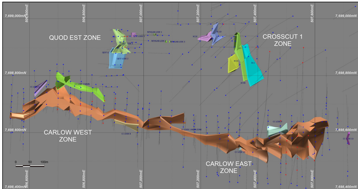
Figure 39: Plan view of the various lodes for the Carlow system, which is currently in progress.
