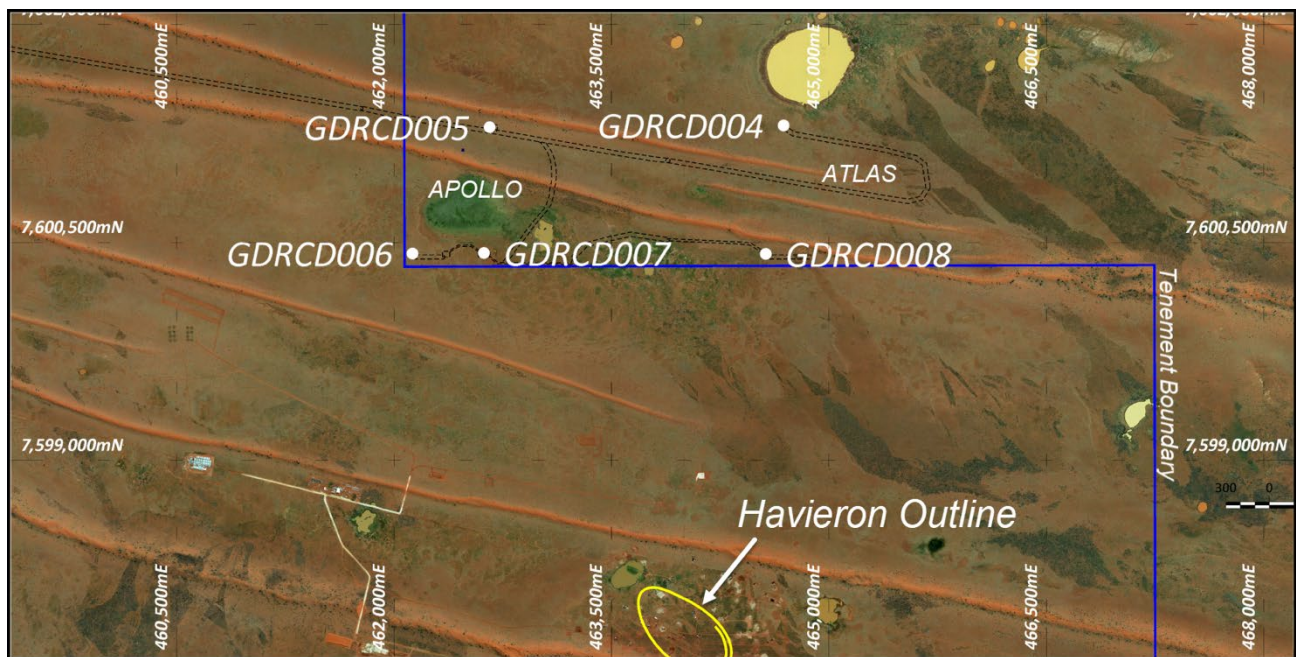
Figure 4: Location of drill collars at Apollo and Atlas in relation to the Haveron deposit.
