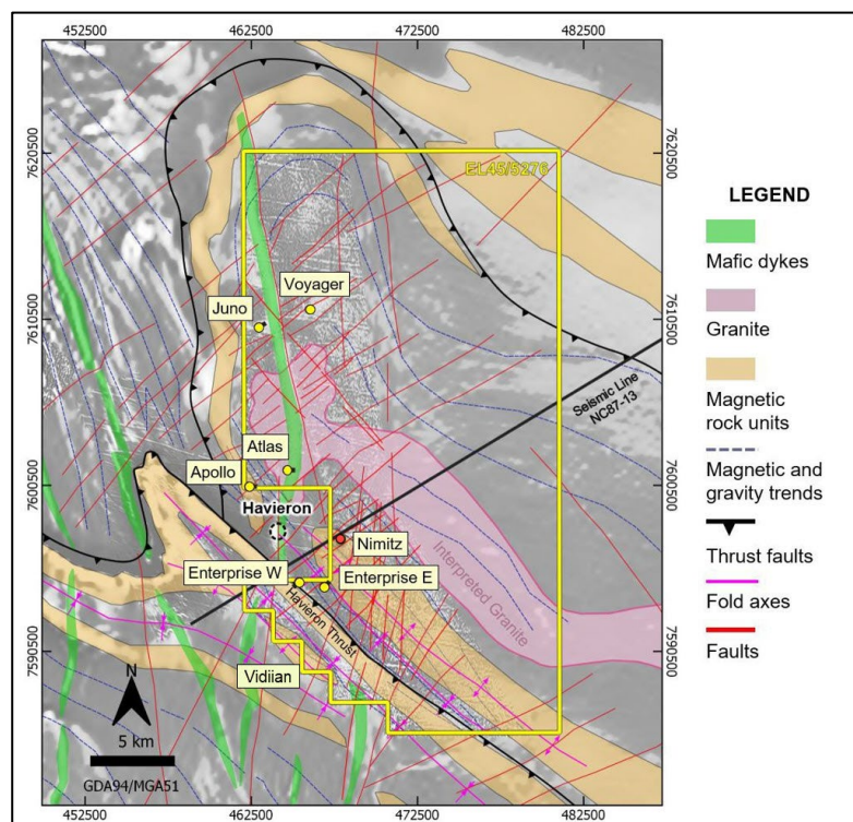
Figure 3: Paterson Central Tenement E45/5276 (yellow outline), interpreted bedrock geology units and structures, on top of a merged magnetic anomaly image and location of 2D seismic reflection survey line. Nimitz Prospect as marked as red, was previously drilled in 2020.
