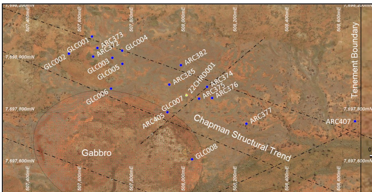
Figure 31: Location of drill collars and simplified geology for the Chapman Prospect. Direction of drill label does not reflect the drill direction. Q3 2021 drilling is prefixed GLC, Q1 2022 drilling prefixed ARC.
