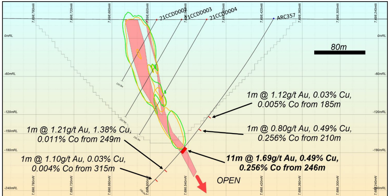
Figure 23: Hole ARC357 Section 507570mE showing the wide interval of mineralisation below the 2021 optimised pit. The line traces highlight the low grade halo with orange outlining the >0.25\text{g/t Au} trace and green outlining >0.25\% Cu as defined by implicit modelling. Refer to Figure 11 for location of the section.
