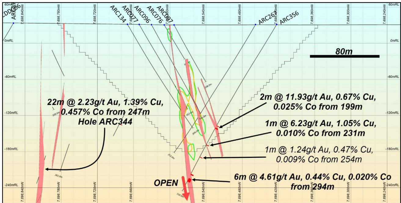
Figure 21: Hole ARC356 Section 507400mE showing significant intersections well below the 2021 optimised pit outline, with mineralisation open at depth. This section of the East Zone is near the Crosscut Zone, as shown by the significant intersection in hole ARC344. The line traces highlight the low grade halo with orange outlining the >0.25g/t Au trace and green outlining >0.25% Cu as defined by implicit modelling. Refer to Figure 11 for location of the section.
