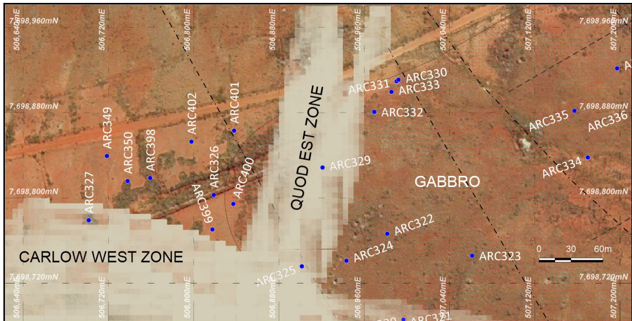
Figure 30: Drill collar locations for the drilling at Quod Est Zone.
