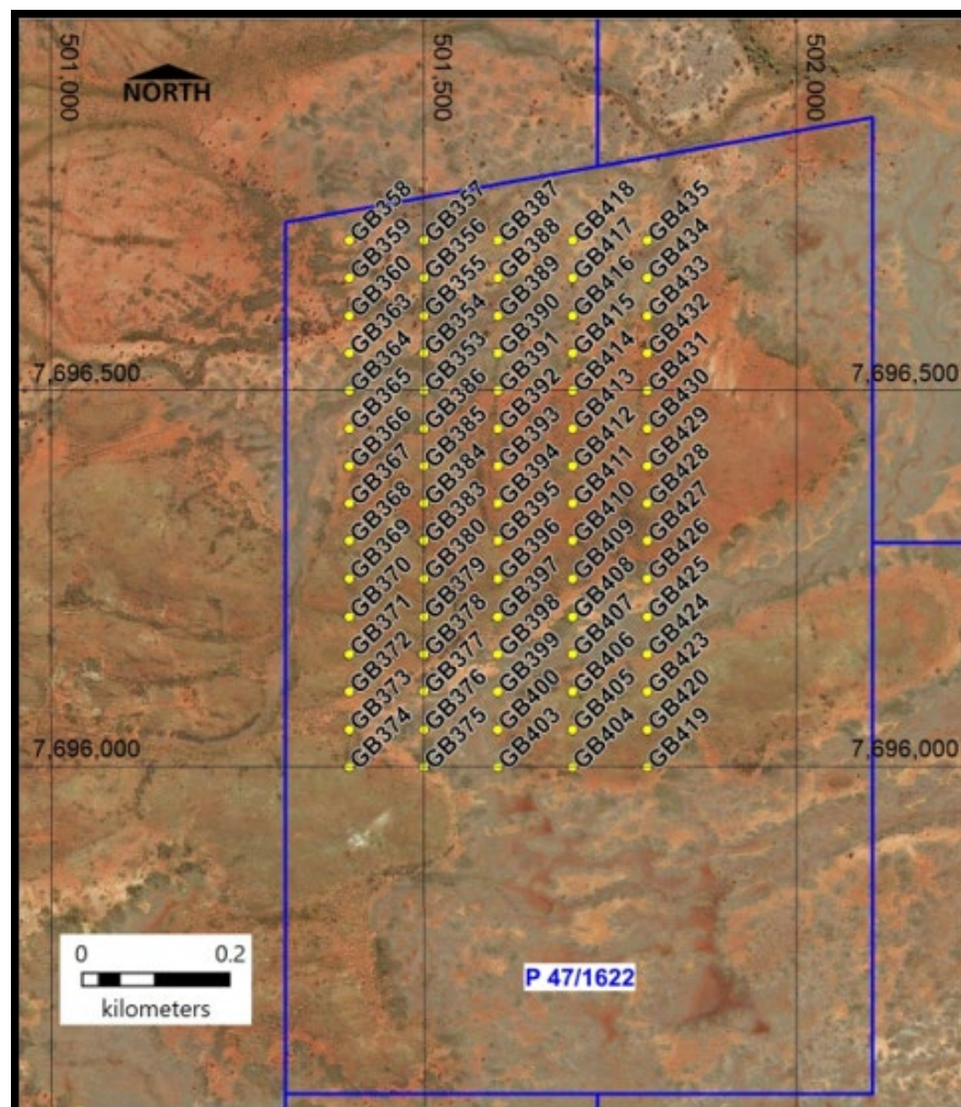
Figure 37: Soil sampling localities on tenement P47/1622. Location of the tenement is shown in Figure 7.
