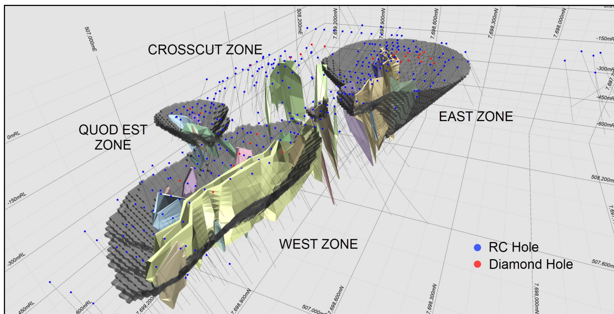
Figure 25: Oblique view of the Carlow System looking northeast, displaying its typical vein splay. New shoot developments occur on the western side of the East Zone pit. Further drilling is required to extend these systems along strike and down dip. Grid scale is approximately 300m.
