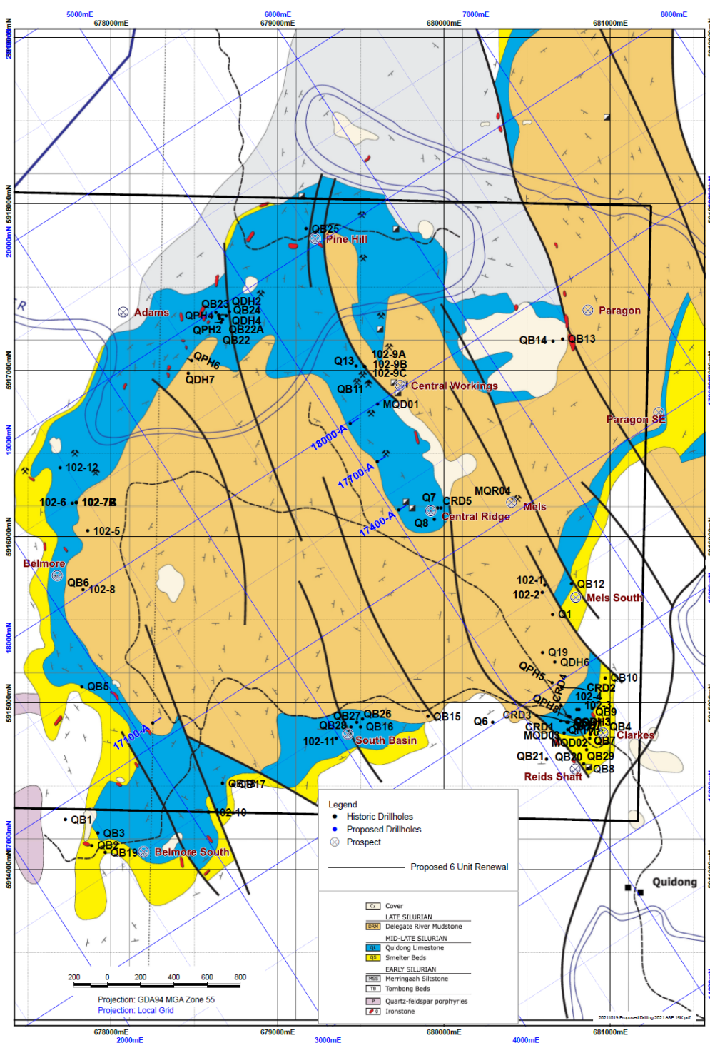
Figure 11: Quidong Basin Geology & Prospects After McQueen 1983; showing planned drillsites in blue
