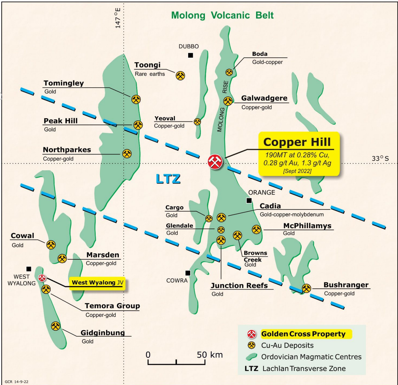
Figure 2: Regional setting of Copper Hill Project
