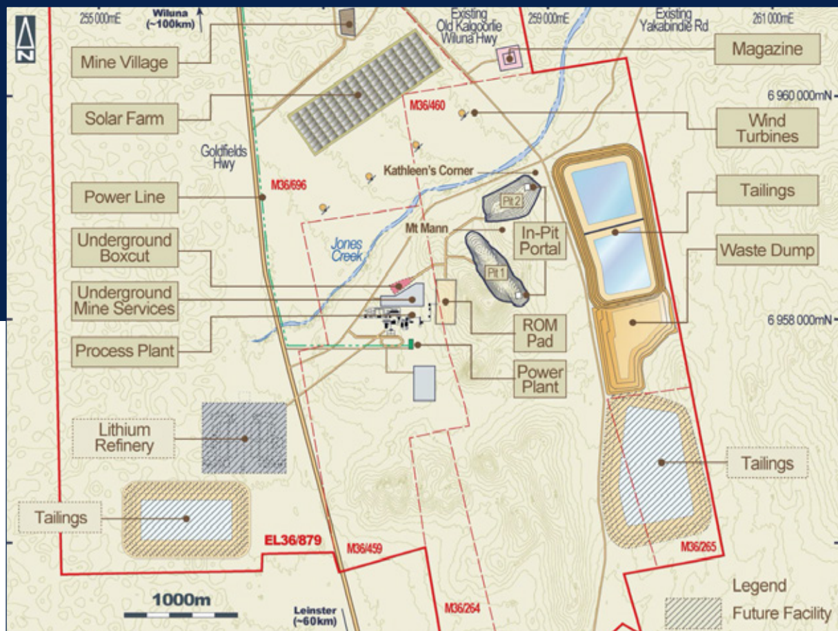
Figure 2: Kathleen Valley Project – Proposed mine site layout
