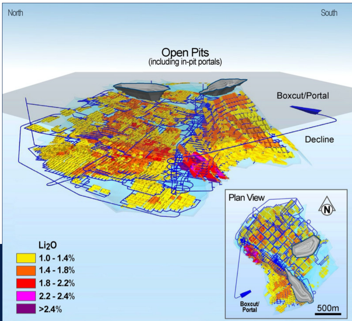
Figure 3: Proposed DFS mine development showing ore stopes by grade
