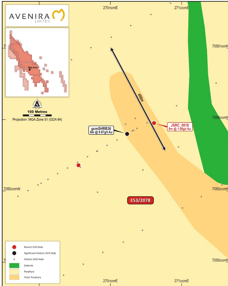
Figure 10. Plan showing intercepts adjacent to JSRC_0018 and existing drilling over Geological Interpretation
