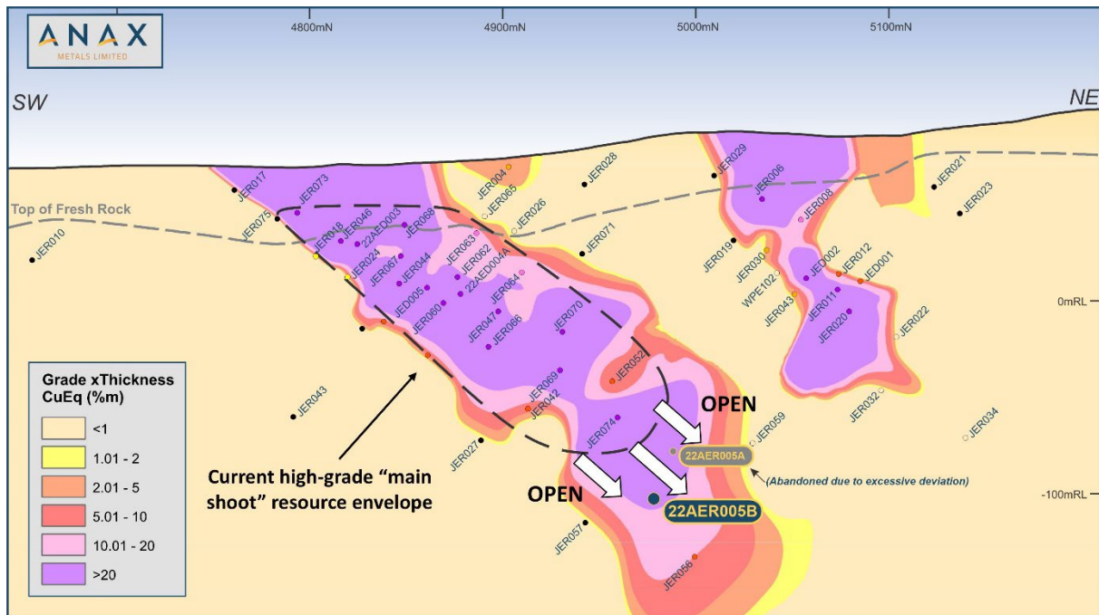
Figure 9: Evelyn Long Section (local grid) showing CuEq grade x thickness contours and drilling pierce points. View direction is to the northwest 34
