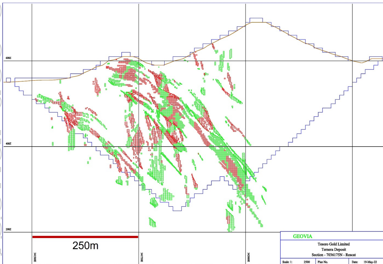
Figure 3 – Ternera Gold Deposit Block Model Section 7036175N (looking north) showing MRE block model and US$1,800/oz optimised open pit shell. Red = indicated classification, green = inferred classification
