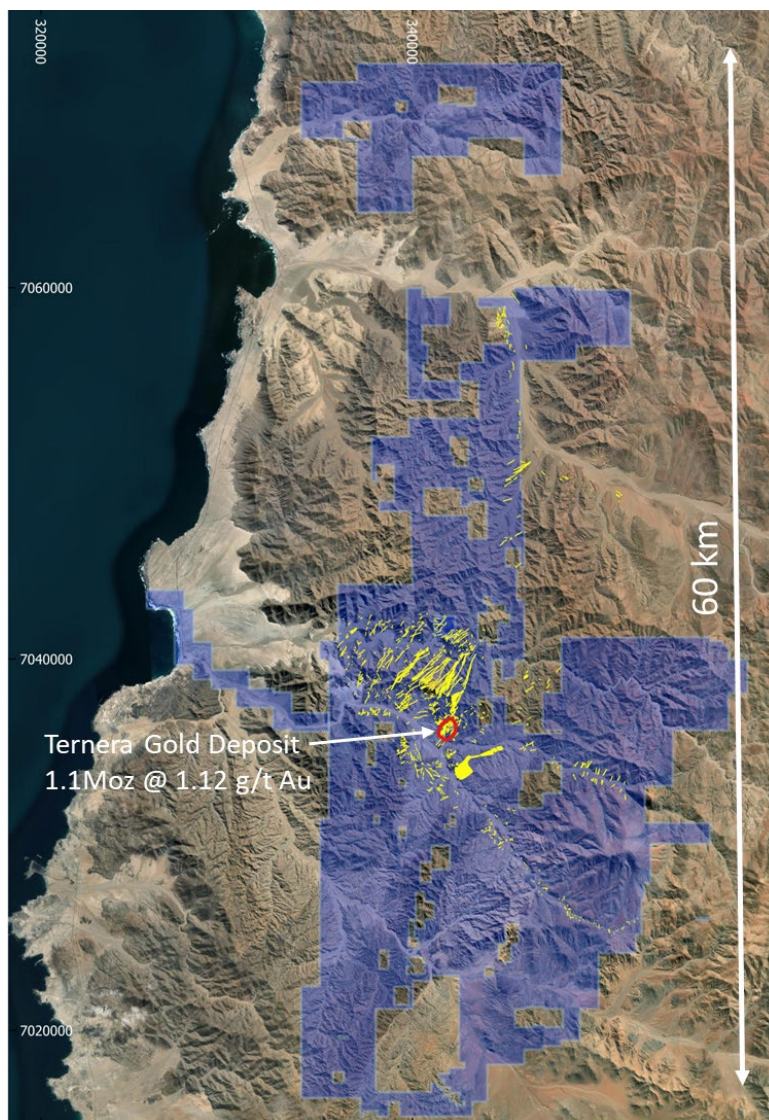
Figure 6 – El Zorro Gold Project Concession Area (blue). Yellow indicates mapped surface outcrop of El Zorro Tonalite bodies, the main gold host rock at El Zorro. Datum PSAD56 19.S
