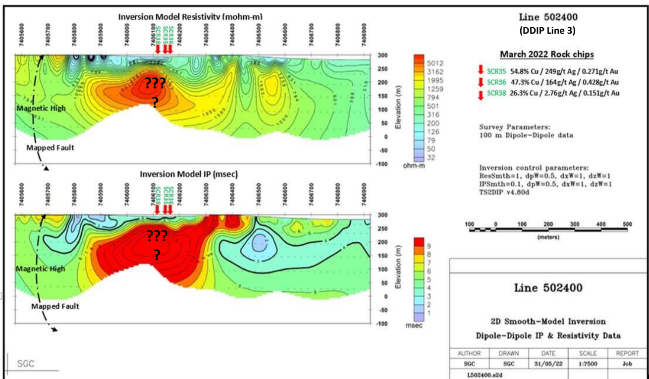
Figure 1: Dipole-Dipole IP line 502400mE (Line 3) TA1 target.
